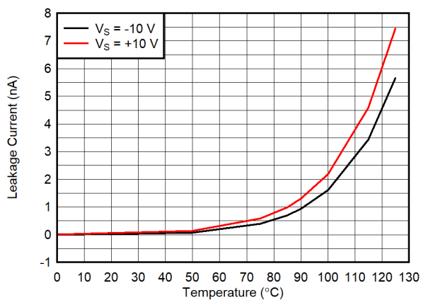
图 6-14. I_{ON} Leakage Current vs Temperature
