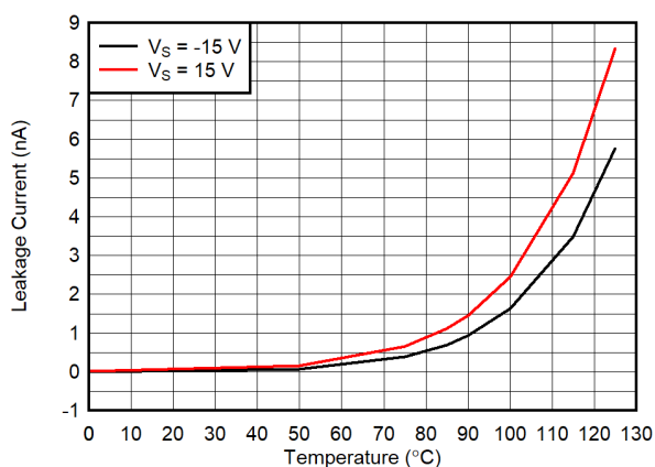
图 6-16. I_{ON} Leakage Current vs Temperature
