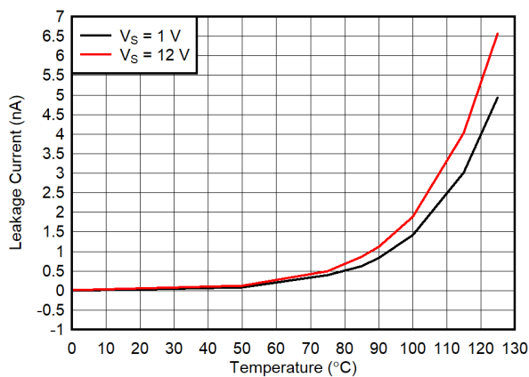
图 6-13. I_{ON} Leakage Current vs Temperature
