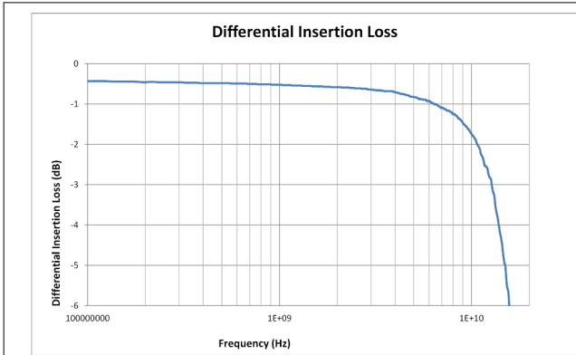
图 5-1. S-Parameter Plots for a TMUXHS4412 Channel: Differential Insertion Loss
