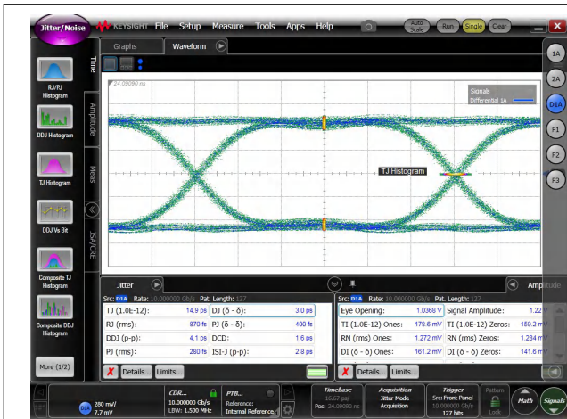
图 5-3. Jitter Decomposition of 10Gbps PRBS-7 Signals in TI Evaluation Board Through Calibration Traces
