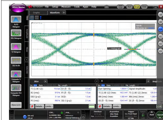
图 7-6. 16Gbps PRBS-7 Signals in TI Evaluation Board Through Calibration Traces
