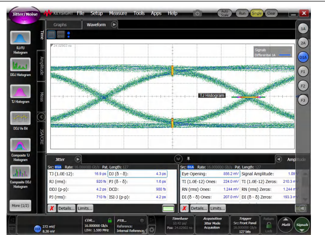
图 7-7. 16Gbps PRBS-7 Signals in TI Evaluation Board Through a Typical TMUXHS4412 Channel
