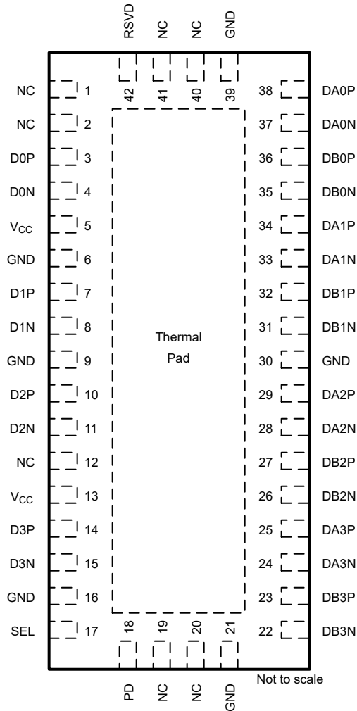
图 4-1. RUA Package 42-Pin WQFN Top View
