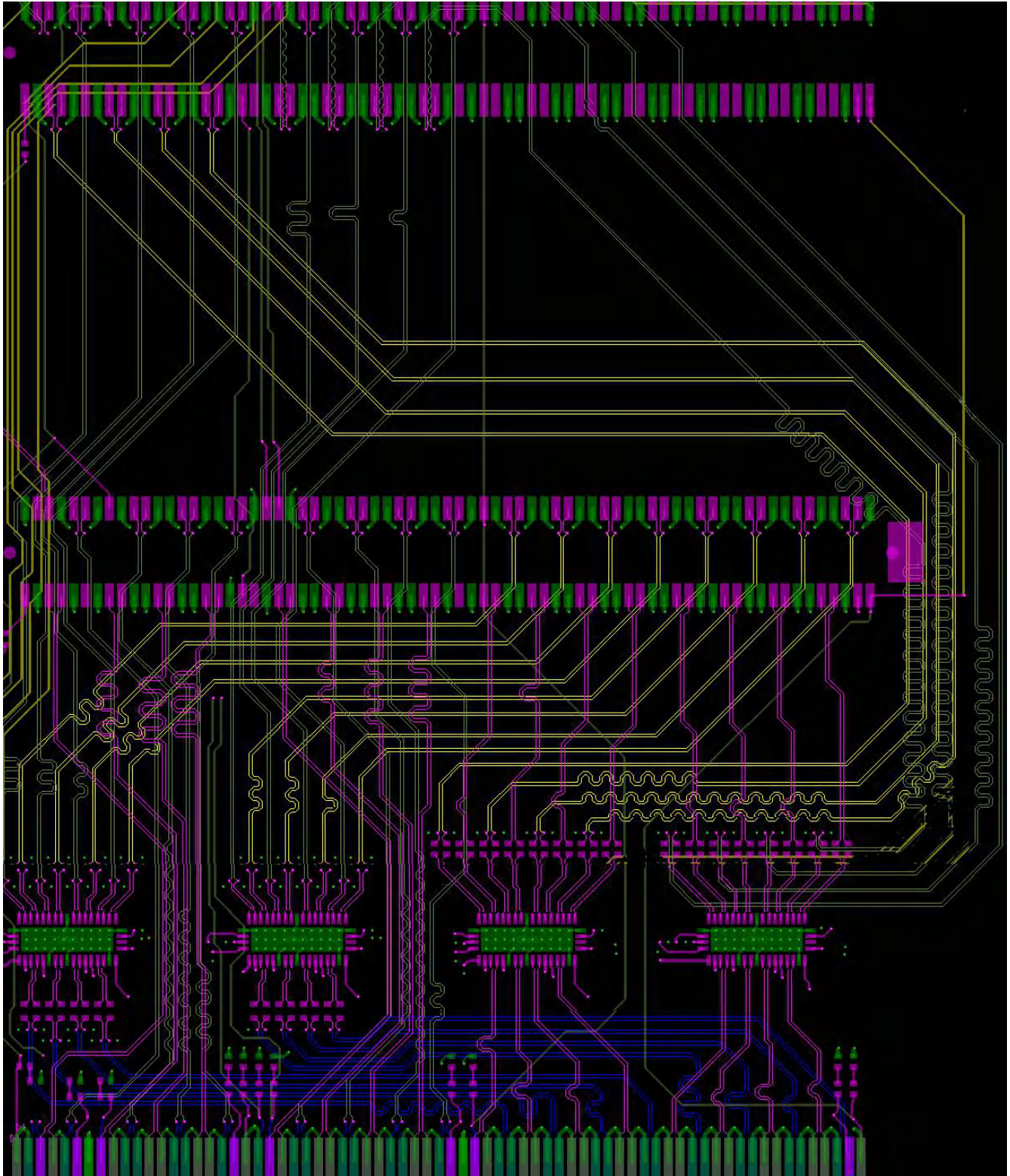
图 7-12. Layout Example for PCIe Lane Muxing Application
