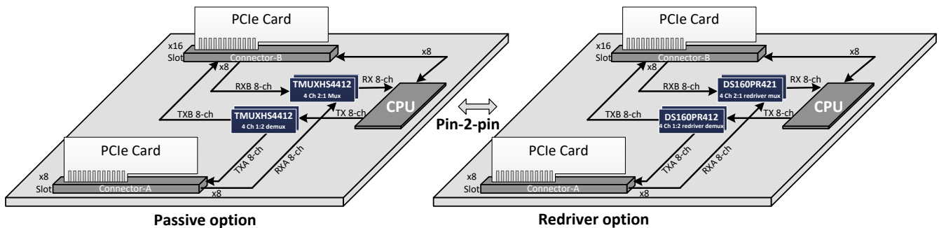
图 7-3. Pin-to-Pin Passive vs Redriver Option for PCIe Lane Switching
