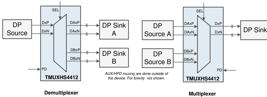
图 7-9. DisplayPort Main Link Demuxing/Muxing
