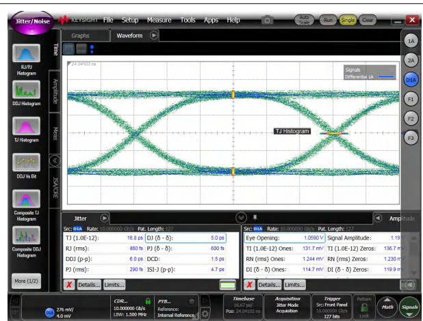
图 5-4. Jitter Decomposition of 10Gbps PRBS-7 Signals in TI Evaluation Board Through a Typical TMUXHS4412 Channel
