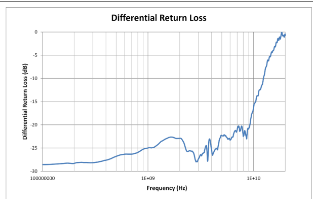
图 5-2. S-Parameter Plots for a TMUXHS4412 Channel: Return Loss vs Frequency
