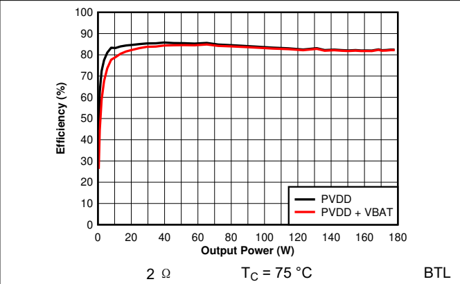
图 6-56. Efficiency vs Output Power - 2 \Omega
