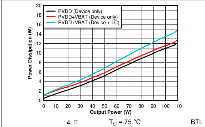
图 6-55. Power Dissipation vs Output Power - 4 \Omega
