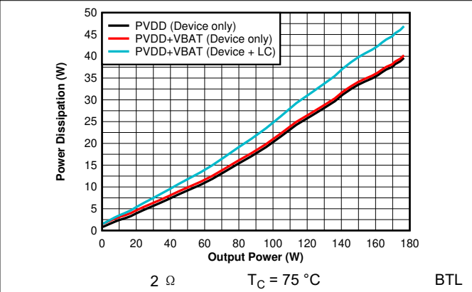
图 6-46. Power Dissipation vs Output Power - 2 \Omega
