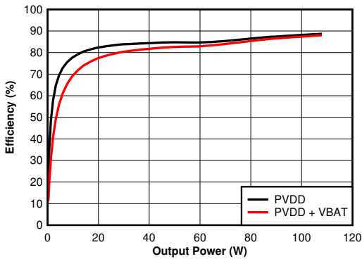
图 6-5. Efficiency vs Output Power - 4 Ω
