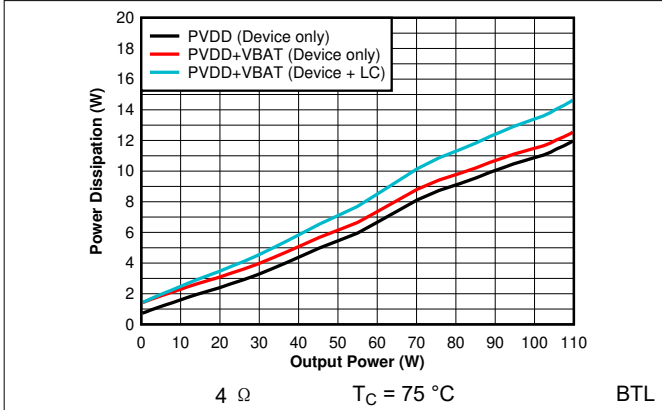
图 6-43. Power Dissipation vs Output Power - 4 \Omega
