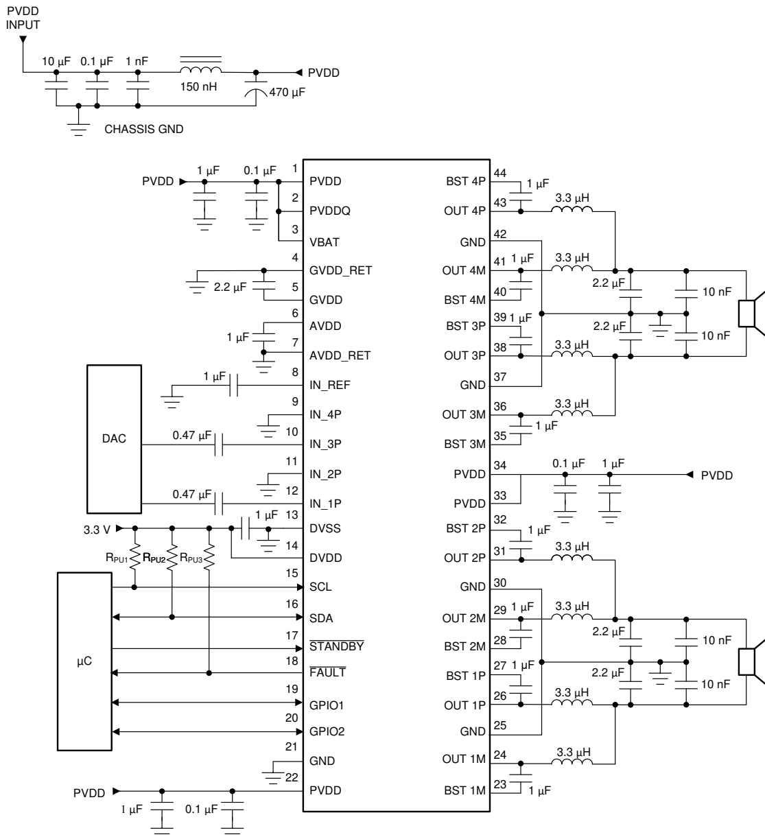
图 8-3. 2-Channel PBTB Application Schematic
