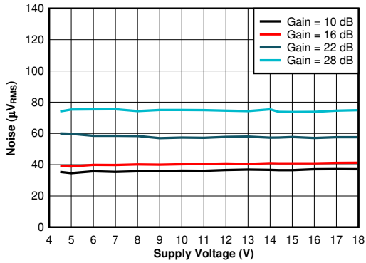
图 6-13. Noise vs Supply Voltage
