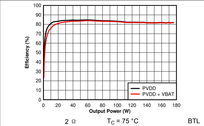
图 6-44. Efficiency vs Output Power - 2 \Omega
