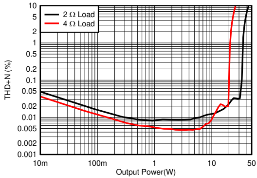
图 6-1. THD+N vs Power - 2 Ω, 4 Ω - 14.4 V
