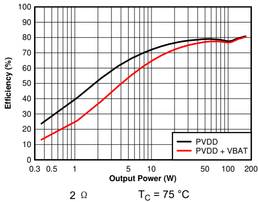
图 6-9. Efficiency vs Output Power - 2 \Omega (Zoomed)
