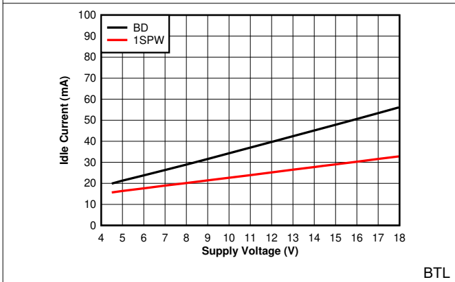
图 6-47. PVDD Idle vs Supply Voltage
