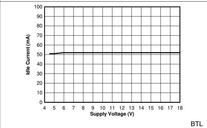
图 6-48. VBAT Idle Current vs Supply Voltage
