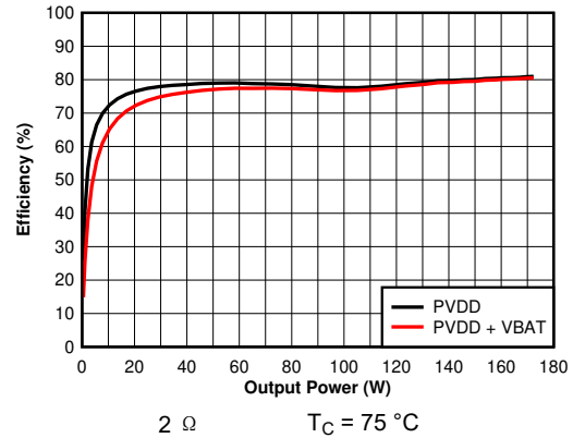
图 6-8. Efficiency vs Output Power - 2 \Omega
