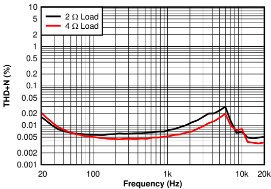
图 6-3. THD+N vs Frequency - 2 Ω, 4 Ω
