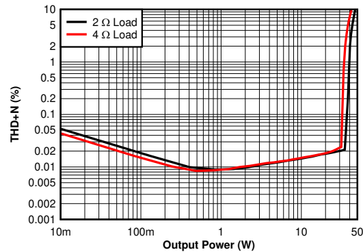
图 6-38. THD+N vs Power - 2 \Omega , 4 \Omega - 18 V
