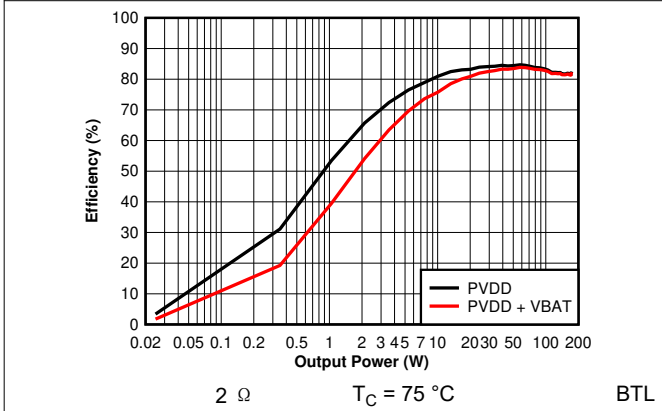
图 6-45. Efficiency vs Output Power - 2 \Omega (Zoomed)
