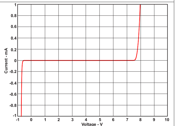
Figure 6. IV Curve On Signal Pins
