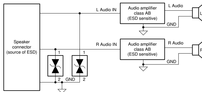
图 8-1. Typical Application Schematic
