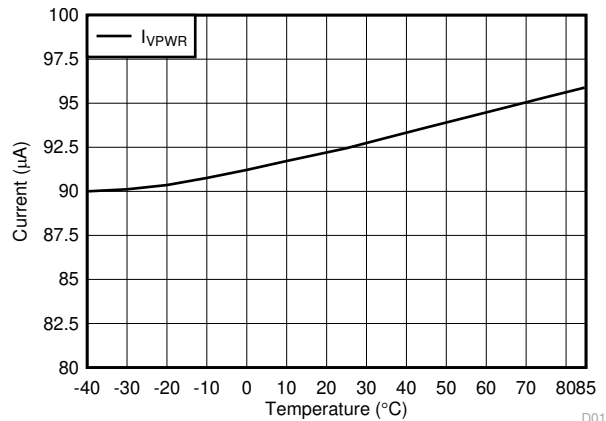
图 7-30. V PWR Supply Leakage vs Ambient Temperature at 3.6 V
