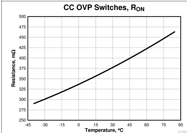
图 7-21. CC R ON Versus Temperature
