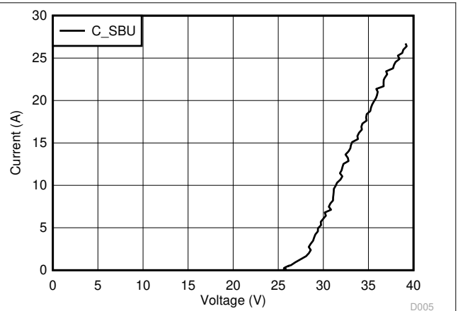
图 7-14. C_SBU TLP Curve Unpowered
