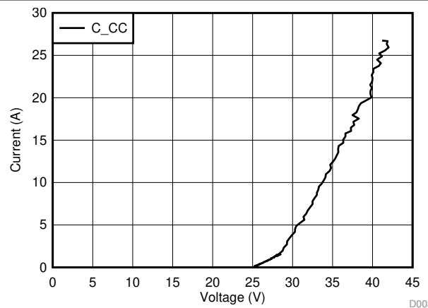
图 7-28. C CC TLP Curve Unpowered
