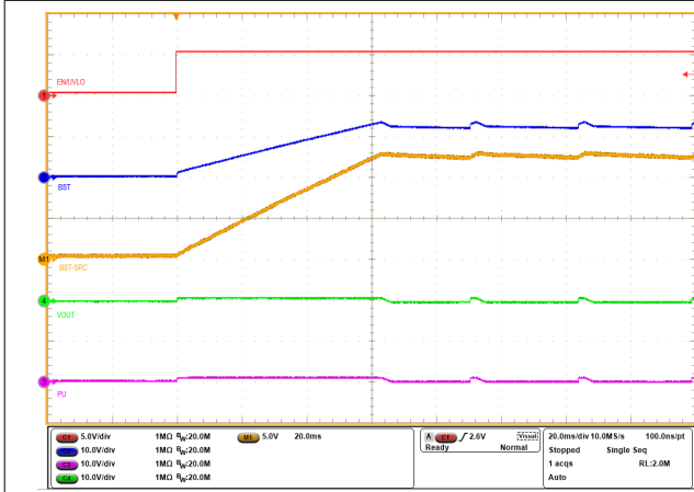
图 8-2. INP = GND 且 C_{BST} = 470\text{nF} 时自举电压的启动曲线
