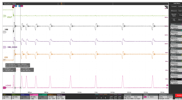
VBB = 13.5V Z OUT1 = 1μH + 100mΩ V EN1 = 5V
