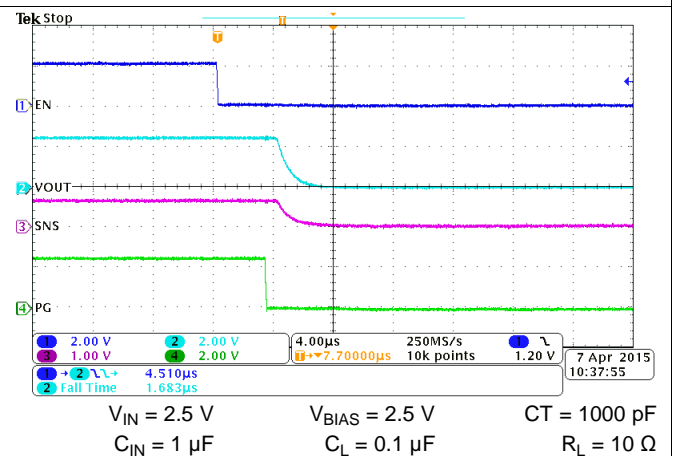
Figure 35. Turn Off Waveform, V_{BIAS} = 2.5 V
