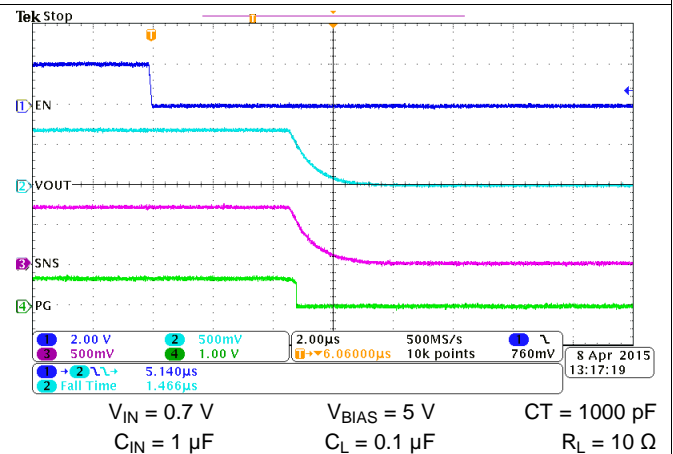
Figure 33. Turn Off Waveform, V_{BIAS} = 5 V
