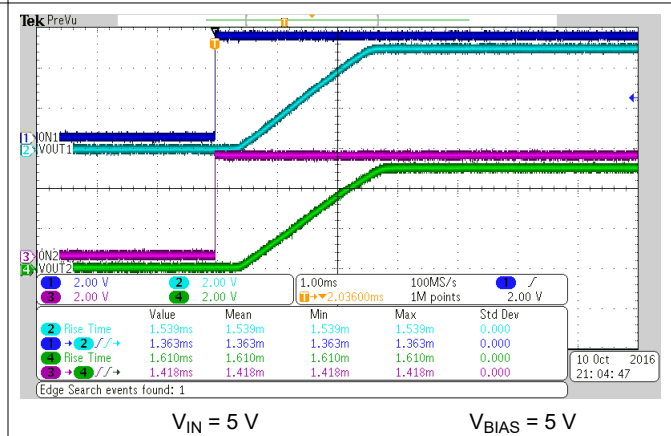
图 6-34. Turnon Response Time
