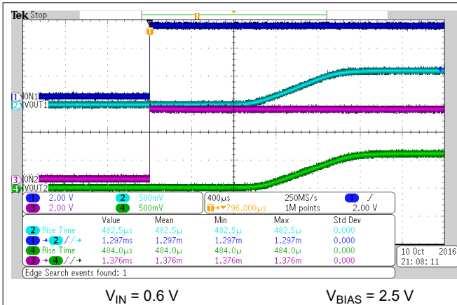
图 6-31. Turnon Response Time
