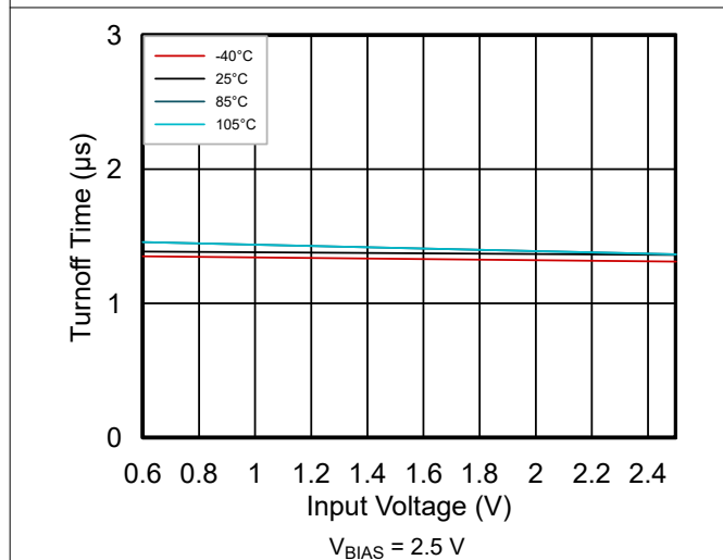
图 6-23. Turnoff Time vs Input Voltage (TPS22976)
