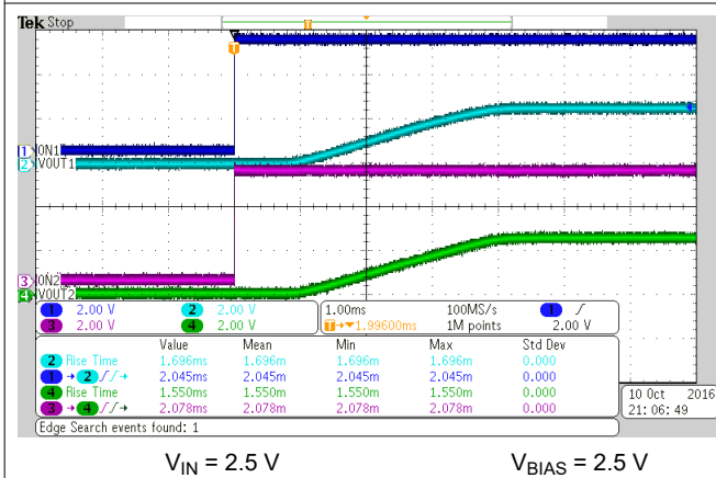
图 6-33. Turnon Response Time
