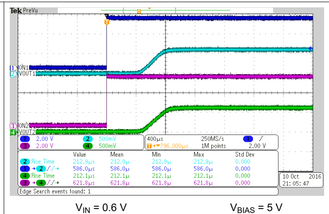
图 6-32. Turnon Response Time
