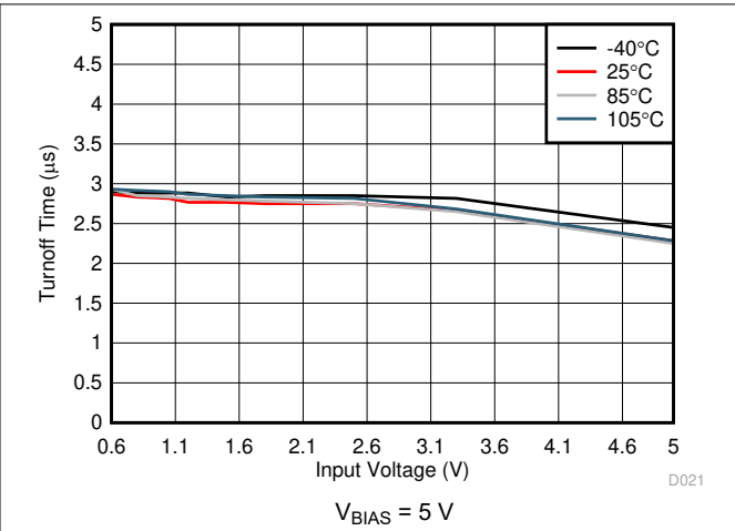
图 6-26. Turnoff Time vs Input Voltage (TPS22976N)
