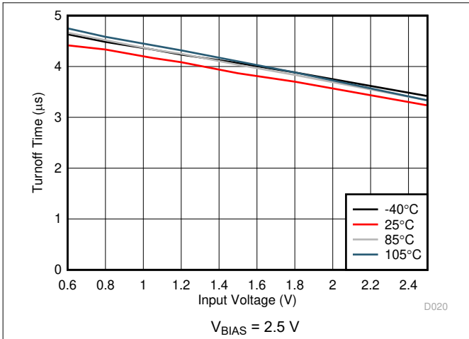
图 6-25. Turnoff Time vs Input Voltage (TPS22976N)
