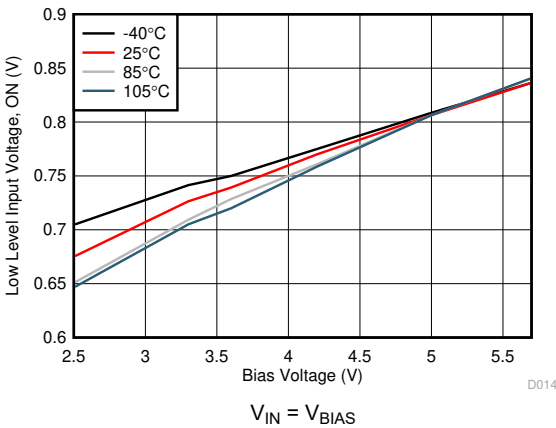
图 6-17. Low-Level Input Voltage vs Bias Voltage
