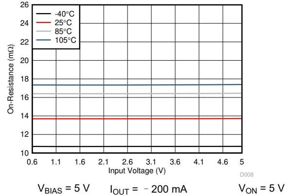
图 6-14. On-Resistance vs Input Voltage Single Channel - Across Ambient Temperatures (TPS22976A, TPS22976N)
