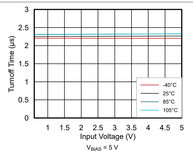
图 6-24. Turnoff Time vs Input Voltage (TPS22976)
