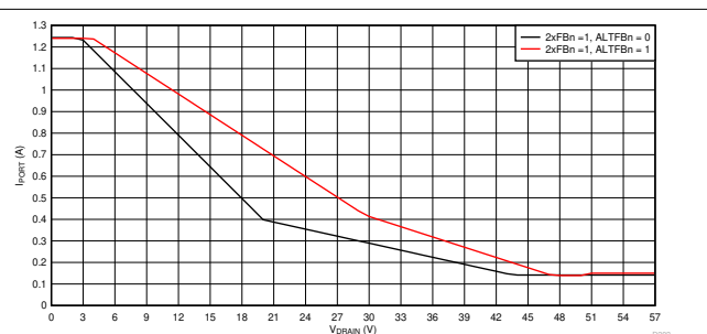
图 9-52. 2x Mode (2xFBn = 1) Foldback Curves, I_{PORT} vs V_{DRAIN}
