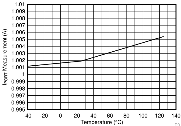
图 7-19. Port Current ADC Measurement (1 A) vs Temperature
