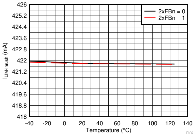
图 7-21. Inrush Current Limit vs Temperature
