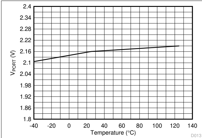
图 7-13. Power Good Threshold vs Temperature
