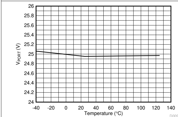
图 7-9. Discovery Open Circuit Voltage vs Temperature
