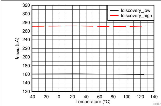
图 7-7. Discovery Currents vs Temperature
