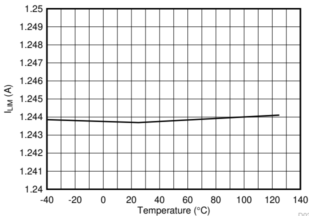
图 7-23. 2x Mode (2xFBn = 1) Current Limit vs Temperature
