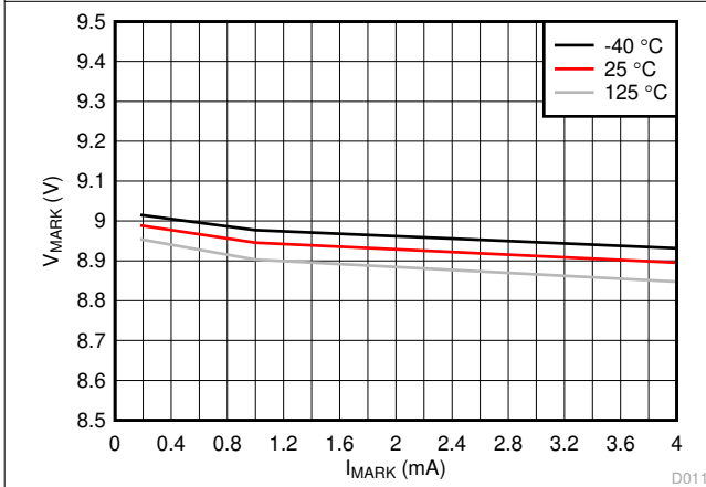
图 7-11. Mark Voltage vs I_{MARK} and Temperature
