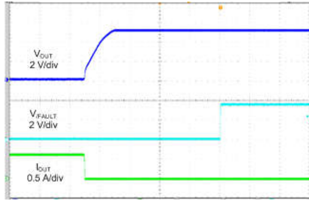
图 6-22. Short Circuit to No Load (SDP)
