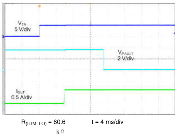
图 6-20. Enable Into Short (SDP)
