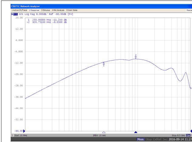
图 6-34. Off-State Data-Switch Isolation vs Frequency
