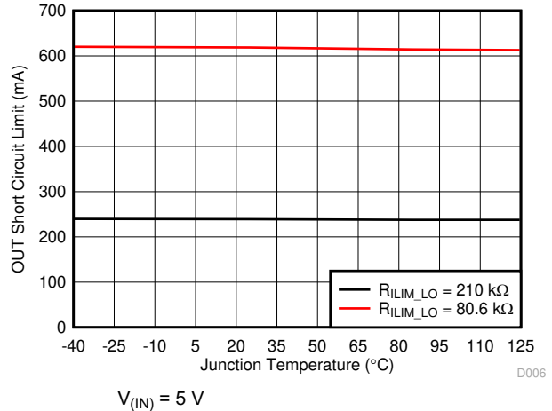
图 6-6. OUT Short-Circuit Current Limit vs Temperature II
