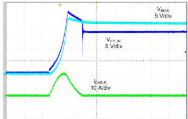
图 9-7. Enabled With OVP_SEL = High, OUT Shorted to Battery
