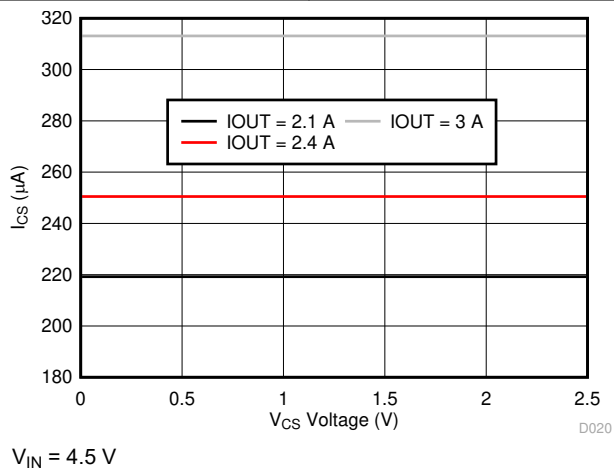
图 6-15. I (IMON) vs V (CS) Voltage
