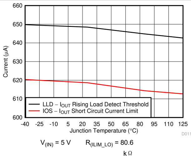
图 6-9. I (OUT) Rising Load-Detect Threshold and OUT Short-Circuit Limit vs Temperature
