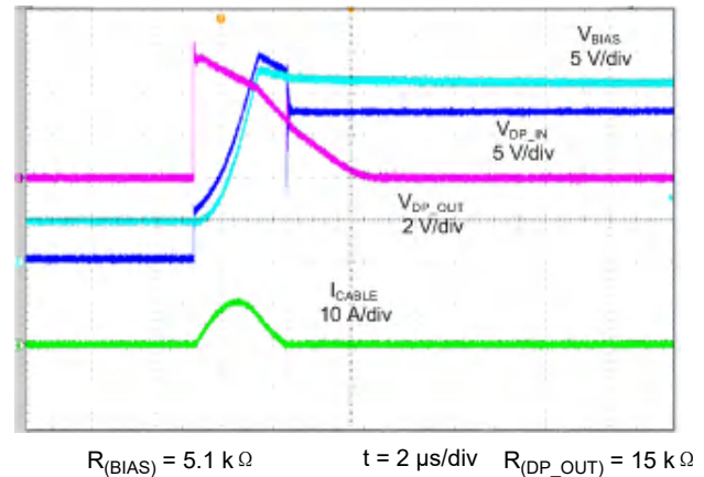
图 9-11. Enabled, DP_IN Shorted to Battery
