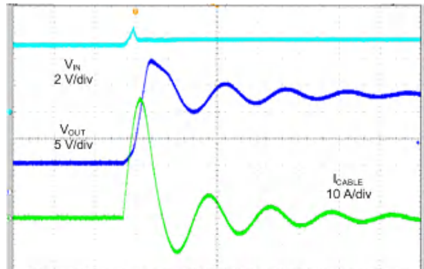
图 9-5. Disabled, 35-V, 1210, X7R C OUT Capacitor With SMAJ18, OUT Shorted to Battery
