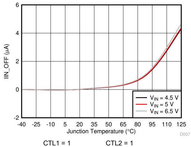
图 6-7. Disabled IN Supply Current vs Temperature
