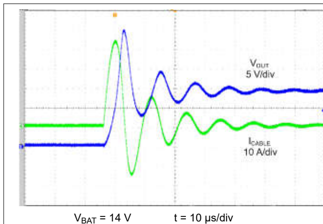
图 9-2. Disabled, 25-V, 1206, X7R C_{OUT} Capacitor Without SMAJ18
