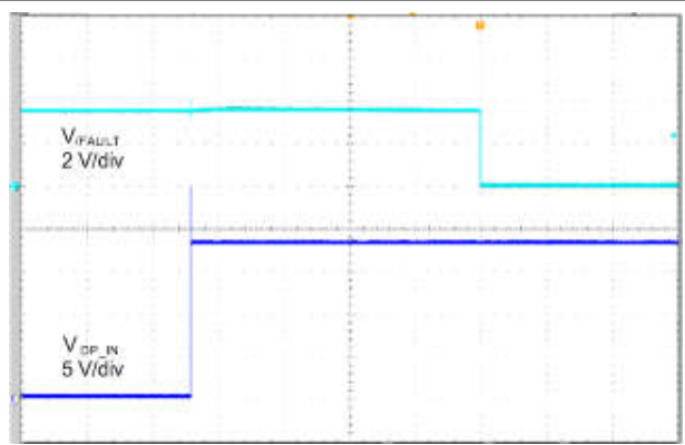
t = 4 \text{ ms/div} 图 6-29. DP_IN Short to Battery
