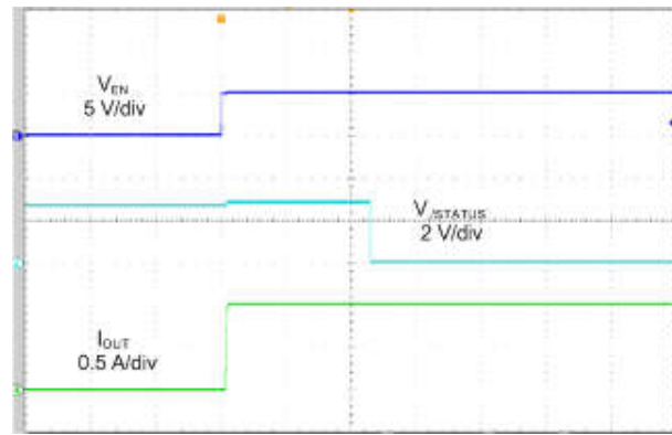
图 6-23. Short Circuit to No Load (CDP)
