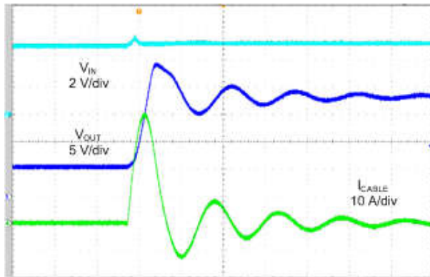
图 9-6. DC-DC Input Is Floating, OUT Shorted to Battery
