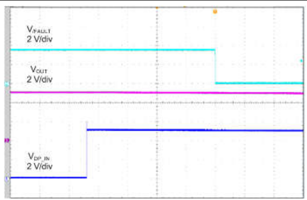
R_{(BIAS)} = 5.1 \text{ k}\Omega t = 4 \text{ ms/div} 图 6-31. DP_IN Short to V_{BUS}
