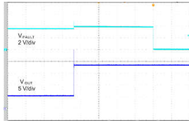
图 6-27. OUT Short to Battery
