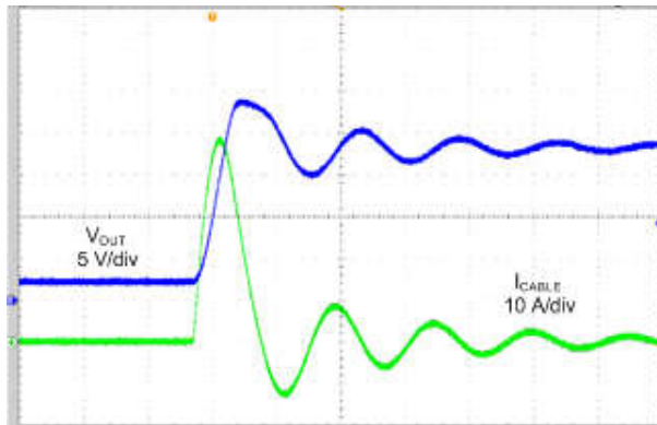
图 9-4. Disabled, 25-V, 1206, X7R C OUT Capacitor With SMAJ18, OUT Shorted to Battery
