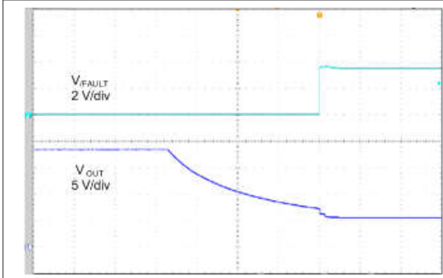
t = 100 \text{ ms/div} 图 6-28. OUT Short-to-Battery Recovery
