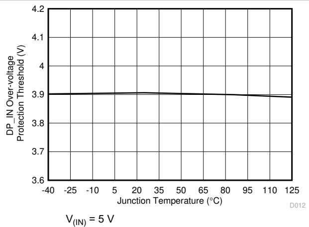
图 6-10. DP_IN Overvoltage Protection Threshold vs Temperature
