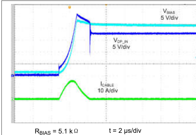
图 9-10. DC-DC Input Is Floating, DP_IN Shorted to Battery
