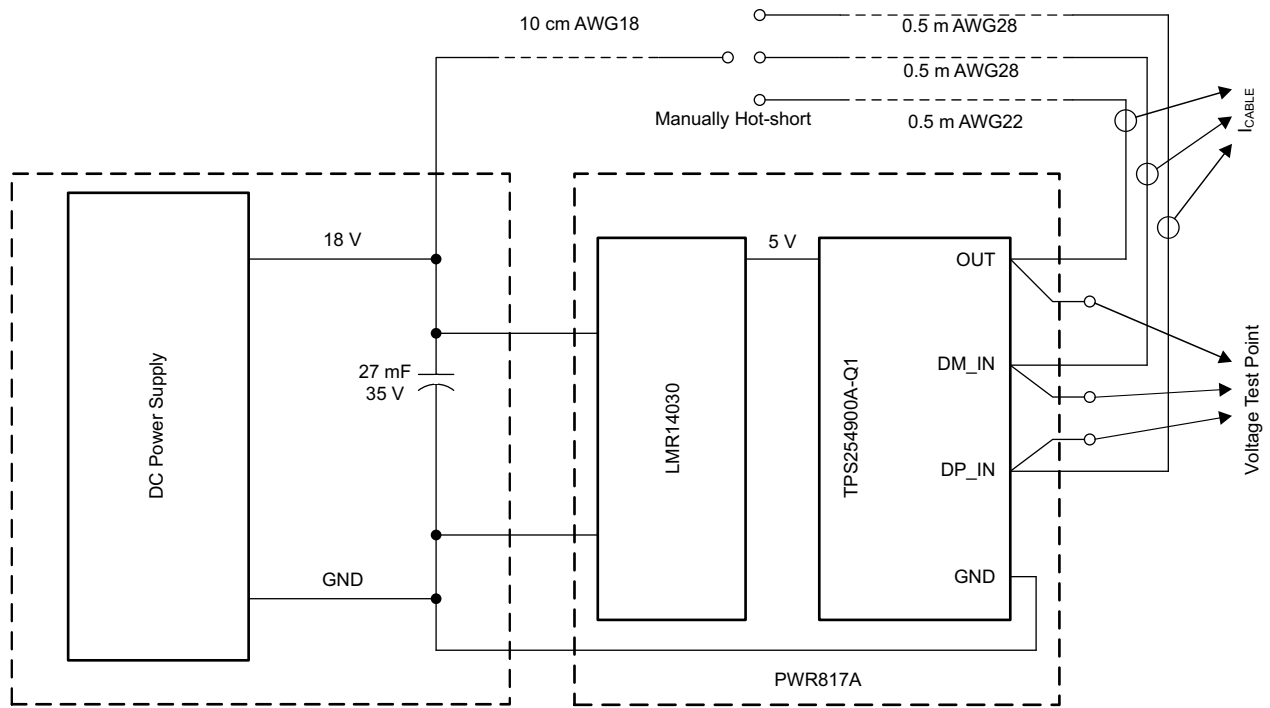
图 7-1. Short-to-Battery System Test Setup
