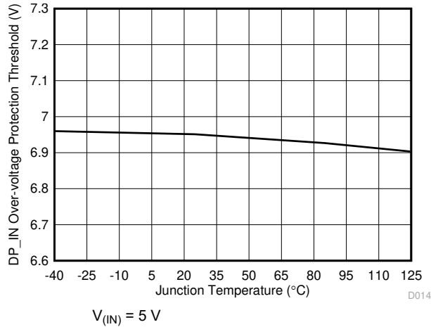
图 6-11. OUT Overvoltage Protection Threshold vs Temperature
