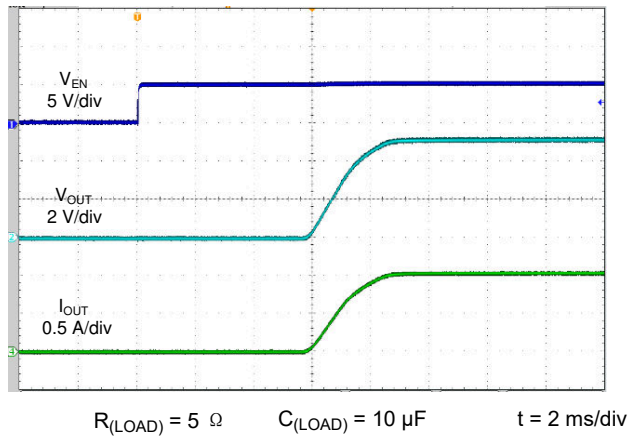
图 6-18. Turnon Response
