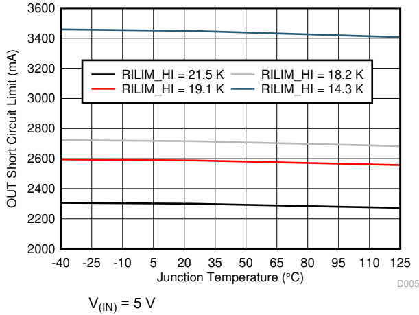
图 6-5. OUT Short-Circuit Current Limit vs Temperature I
