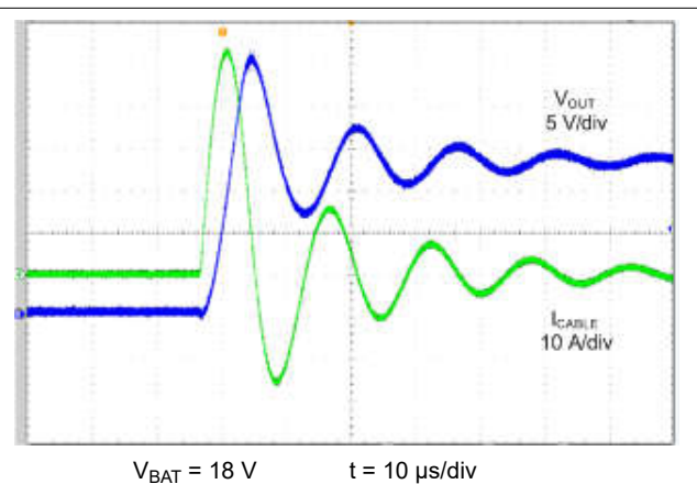
图 9-3. Disabled, 35-V, 1210, X7R C_{OUT} Capacitor Without SMAJ18
