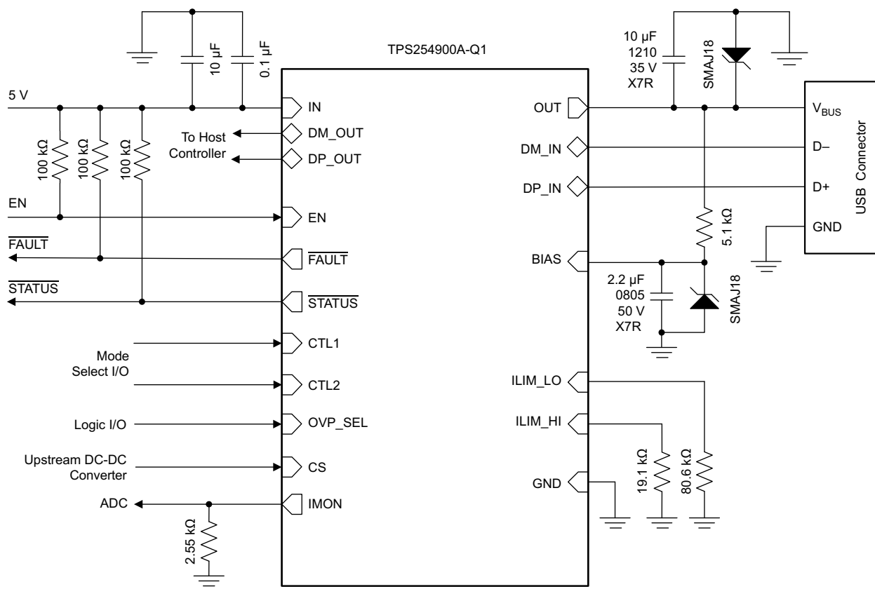
图 9-1. Typical Application Schematic: USB Port Charging With Cable Compensation
