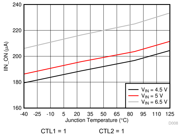
图 6-8. Enabled IN Supply Current - CDP (11) vs Temperature
