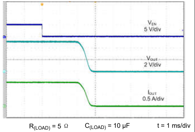
图 6-19. Turnoff Response
