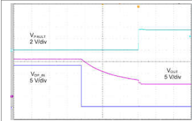
R_{(BIAS)} = 5.1 \text{ k}\Omega t = 100 \text{ ms/div} 图 6-30. DP_IN Short-to-Battery Recovery
