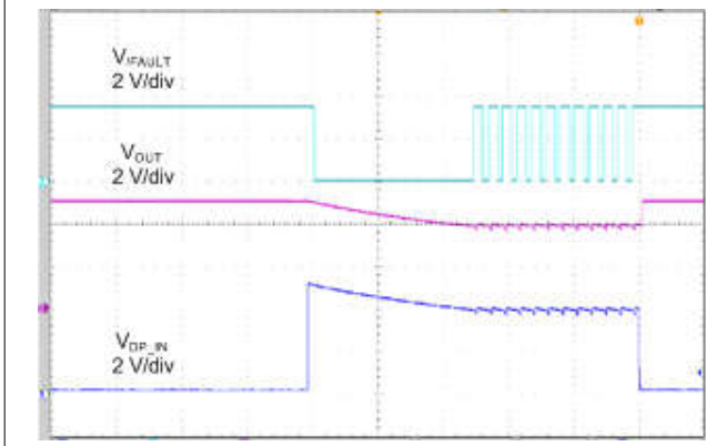
R_{(BIAS)} = 5.1 \text{ k}\Omega t = 200 \text{ ms/div} 图 6-32. DP_IN Short-to- V_{BUS} and Recovery
