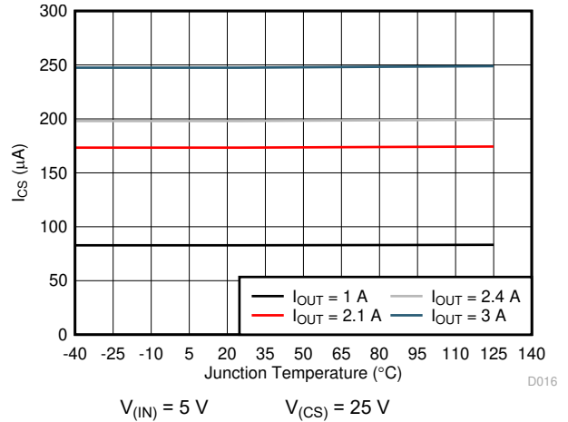
图 6-12. I (CS) vs Temperature
