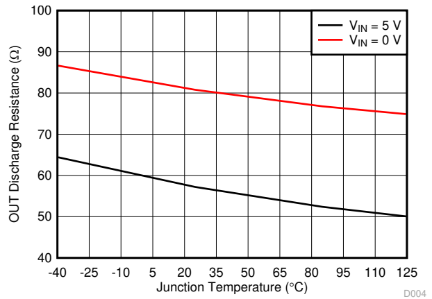
图 6-4. OUT Discharge Resistance (OVP) vs Temperature
