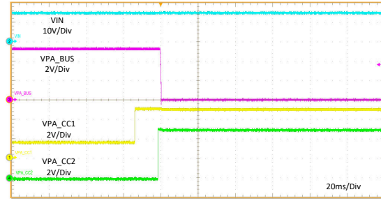
PA_CC1 = R_d to Open PA_CC2 = Open I_{PA\_BUS} = 3\text{ A}
