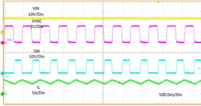
VIN = 13.5 V L = 0.68 uH I PA_BUS = 3 A I PB_BUS = 3 A
