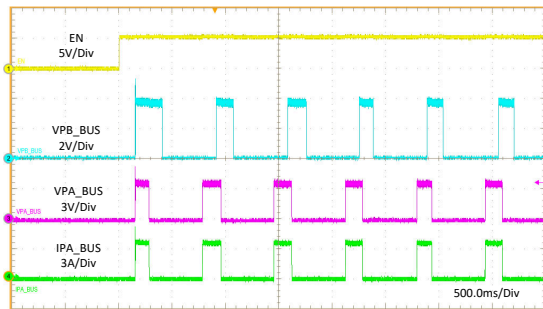
EN to High PA_BUS = 1\ \Omega PB_BUS = 1\ \Omega
