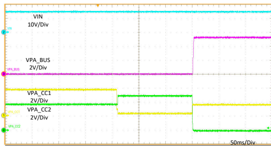
PA_CC1 = Open to R_d PA_CC2 = Open I_{PA\_BUS} = 3\text{ A}
