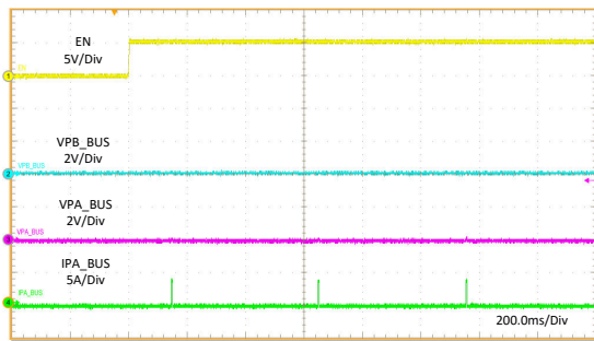
EN to High PA_BUS = GND PB_BUS = GND
