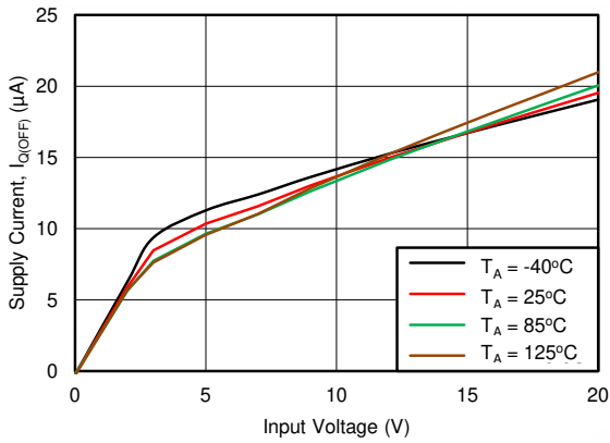
图 7-3. Input Supply Current vs Supply Voltage at Shutdown
