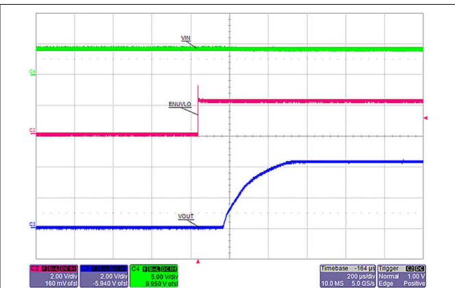
图 7-32. Turn ON with Enable
