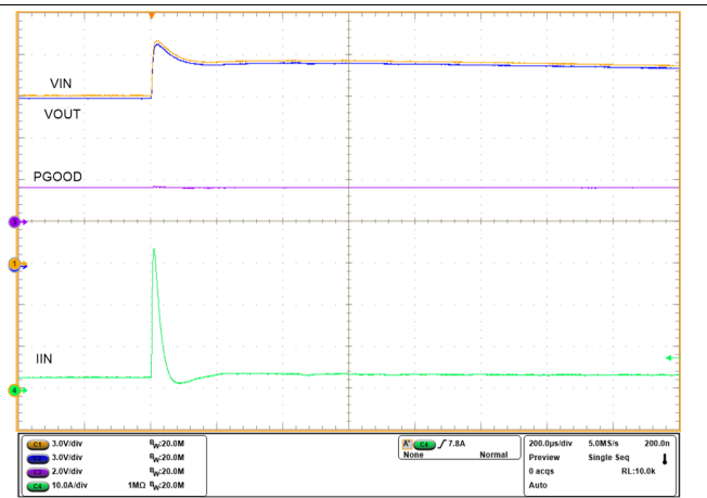
图 40. Supply Line Transient Immunity - Input Voltage Step
