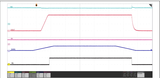
Input supply held steady, EN/UVLO pin held high, SWEN pin toggled high and low 图 7-26. Power Up and Down Sequencing Using SWEN Pin
