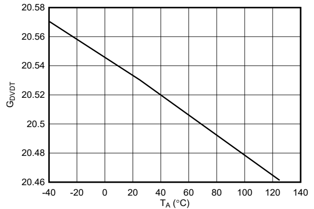
图 7-20. DVDT Gain Across Temperature
