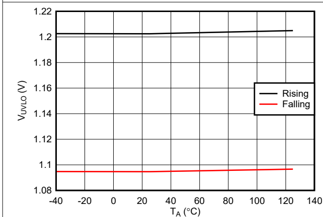
图 7-5. EN/UVLO Thresholds Across Temperature
