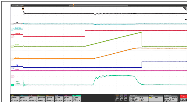
图 9-4. Input Hot Plug: V_{IN} Stepped Up from 0 V to 12 V, C_{LOAD} = 55 mF, C_{DVDT} = 33 nF, R_{IREF} = 40.2 k \Omega , and R_{ILIM} on Each Device = 300 \Omega
