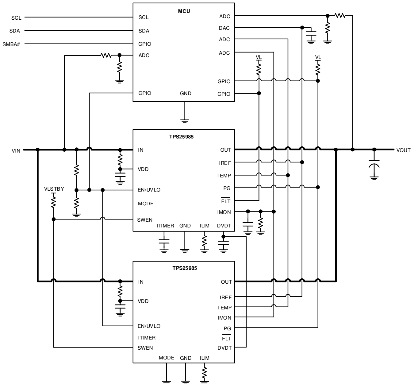
图 9-16. Digital Telemetry Using External Microcontroller
