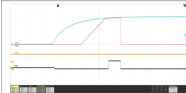
Input supply ramped up above 16.6 V 图 7-29. Input Overvoltage Protection Response
