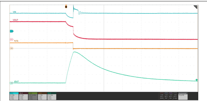
图 7-32. Short-Circuit Protection Response
