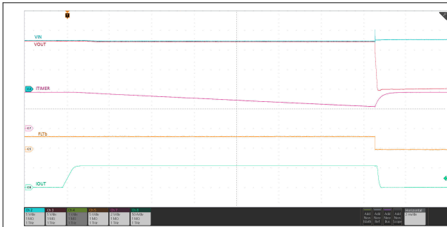
图 7-31. Overcurrent Protection Response (Circuit-Breaker)
