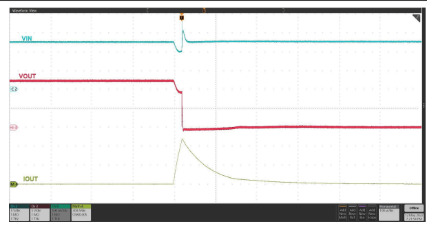
图 9-13. Output Hot-Short Response: V_{IN} = 12\text{ V} , R_{IMON} = 167\ \Omega , R_{REF} = 40.2\text{ k}\Omega , and OUT Shorted to GND
