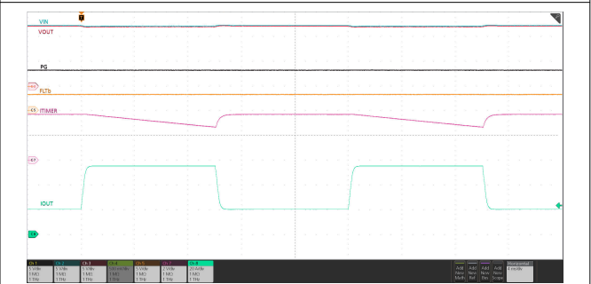
I_{OCP} = 50 \text{ A} , t_{TIMER} = 14 \text{ ms} , I_{OUT} pulsed above the I_{OCP} threshold for short duration without triggering circuit-breaker response 图 7-30. Peak Current Support Using Transient Overcurrent Blanking
