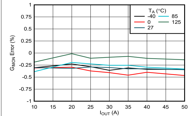
图 7-9. IMON Gain Accuracy Across Load and Temperature
