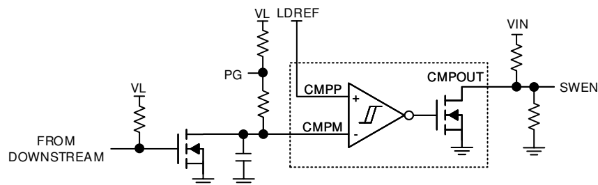
图 8-12. Load Handshake or Detect Timer Using Internal Comparator
