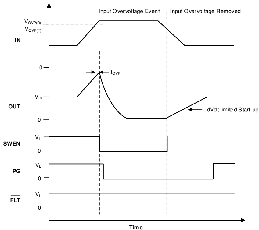
图 8-3. Input Overvoltage Protection Response
