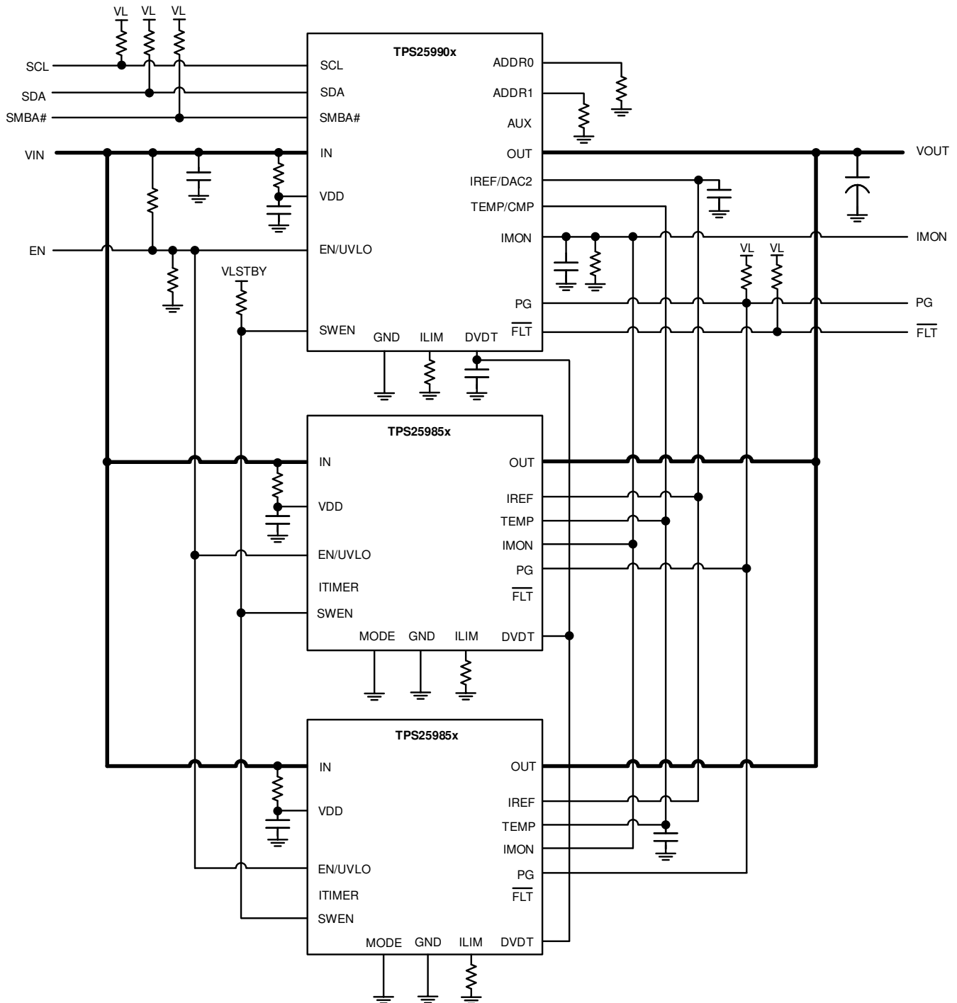
图 9-15. TPS25990x Connected in Parallel with TPS25985x For Higher Current Support With PMBus®
