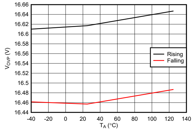
图 7-4. Overvoltage Protection Threshold Across Temperature
