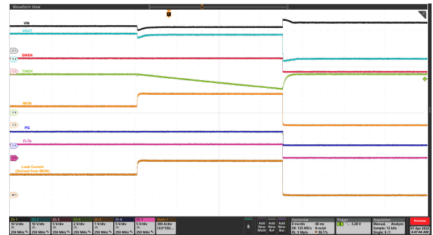
图 9-11. Circuit-Breaker Response: V_{IN} = 12\text{ V} , C_{ITIMER} = 22\text{ nF} , C_{LOAD} = 55\text{ mF} , R_{IMON} = 167\ \Omega , R_{REF} = 40.2\text{ k}\Omega , and Load Current Stepped From 300 A to 500 A for > 20 ms
