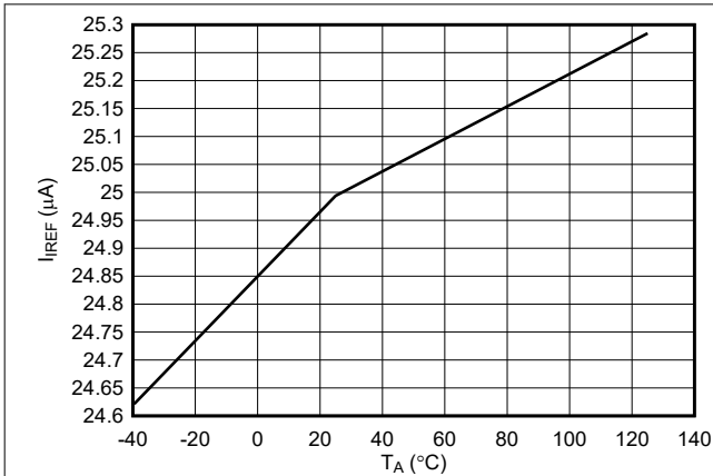
图 7-7. IREF Charging Current Across Temperature
