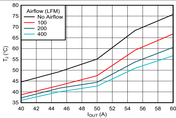
图 7-23. Junction Temperature vs Load Current ( T_A = 25^\circ\text{C} , With Air-Flow)
