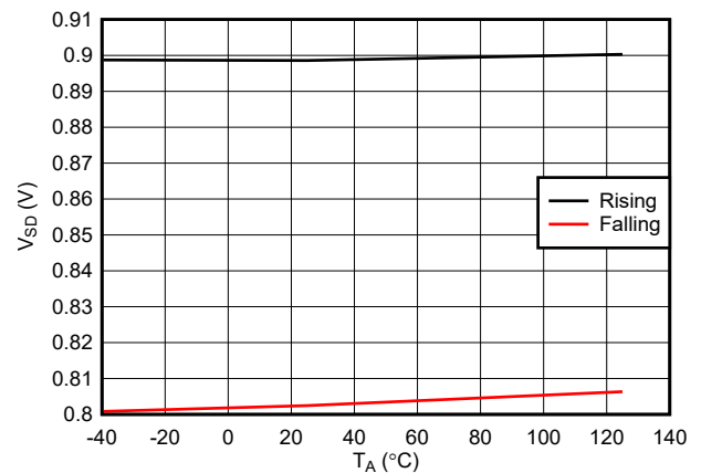
图 7-6. EN/UVLO Based Shutdown Falling Threshold Across Temperature
