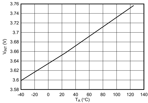
图 7-15. ITIMER Pin Internal Pullup Voltage Across Temperature
