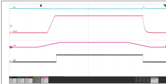
Input supply held steady, EN/UVLO pin toggled high and low 图 7-25. Power Up and Down Sequencing Using EN/UVLO Pin
