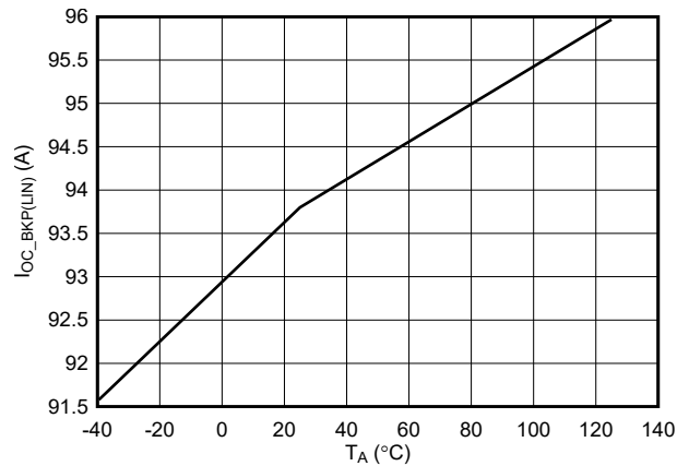
图 7-14. Backup Overcurrent Protection Threshold (Steady-State) Accuracy
