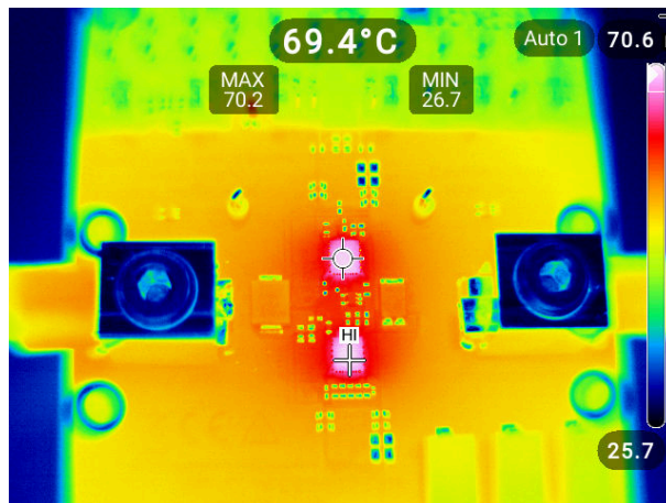
图 9-14. Two (2) TPS25985x eFuses in Parallel: Temperature Rise with 100-A DC Current at Room Temperature (No Air-Flow)
