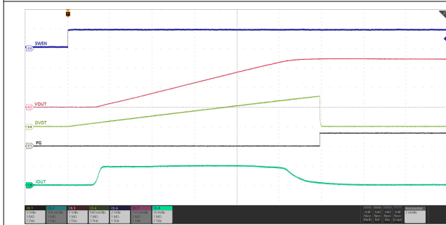
C_{OUT} = 6.8 \text{ mF} , C_{dVdt} = 33 \text{ nF} 图 7-27. Inrush Current Control with Capacitive Load
