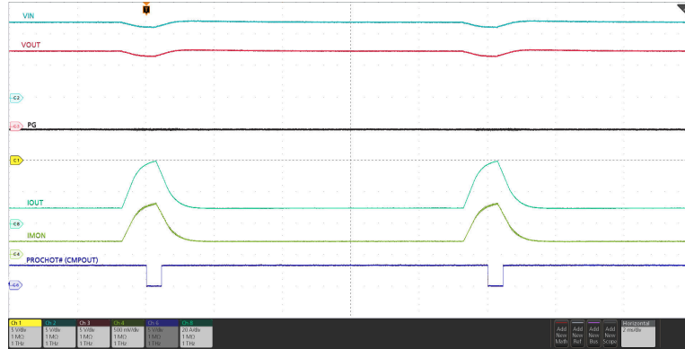
图 8-10. PROCHOT# Response Using Internal Comparator
