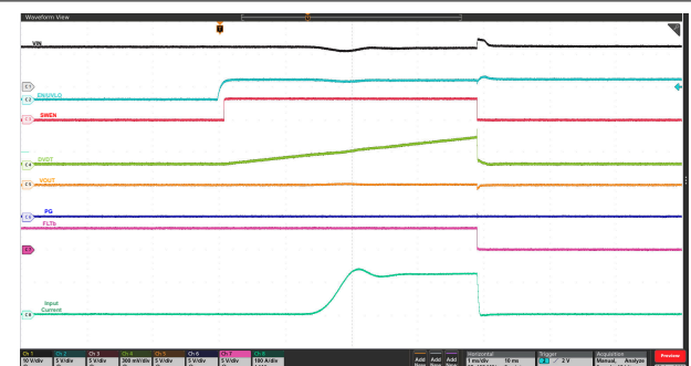
图 9-7. Power Up into Short: V_{IN} = 12 V, EN/UVLO Stepped Up From 0 V to 3 V, R_{IREF} = 40.2 k \Omega , R_{ILIM} on Each Device = 300 \Omega , and OUT Shorted to GND
