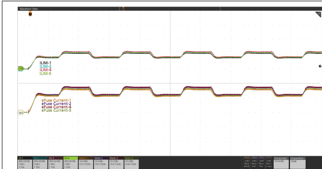
图 9-10. Transient Overload (Current distribution among five devices in parallel): V_{IN} = 12\text{ V} , C_{ITIMER} = 22\text{ nF} , C_{LOAD} = 55\text{ mF} , R_{IMON} = 167\ \Omega , R_{REF} = 40.2\text{ k}\Omega , and Load Current Stepped from 300 A to 450 A then 300 A within 8.5 ms
