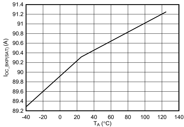
图 7-13. Backup Overcurrent Protection Threshold (Start-up) Accuracy
