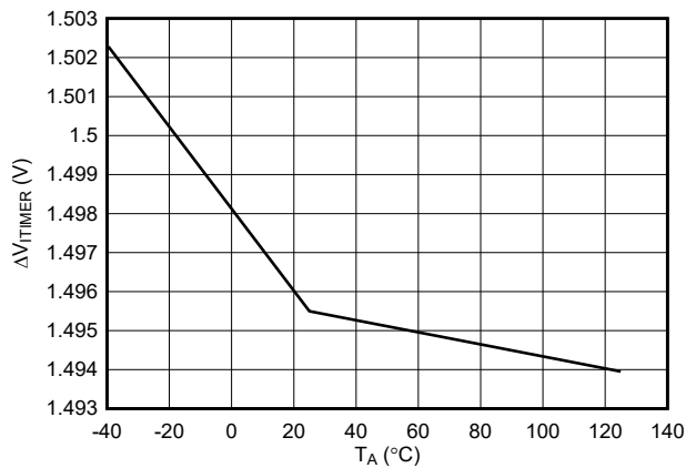
图 7-17. ITIMER Pin Discharge Differential Voltage Threshold Across Temperature
