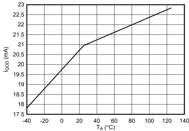
图 7-21. QOD Sink Current Across Temperature
