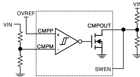
图 8-11. Fast Overvoltage Protection with Adjustable Threshold Using Internal Comparator
