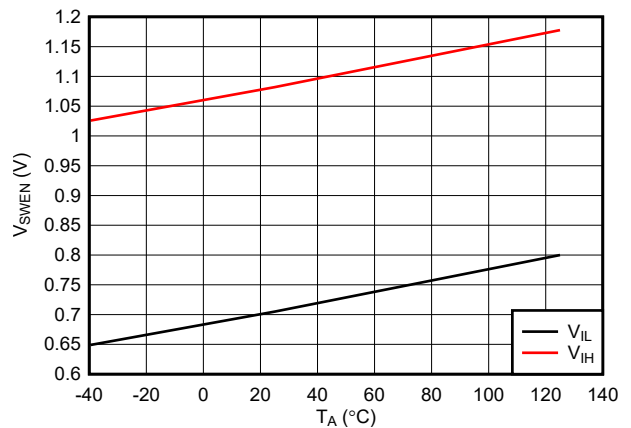
图 7-18. SWEN Pin Logic Thresholds Across Temperature
