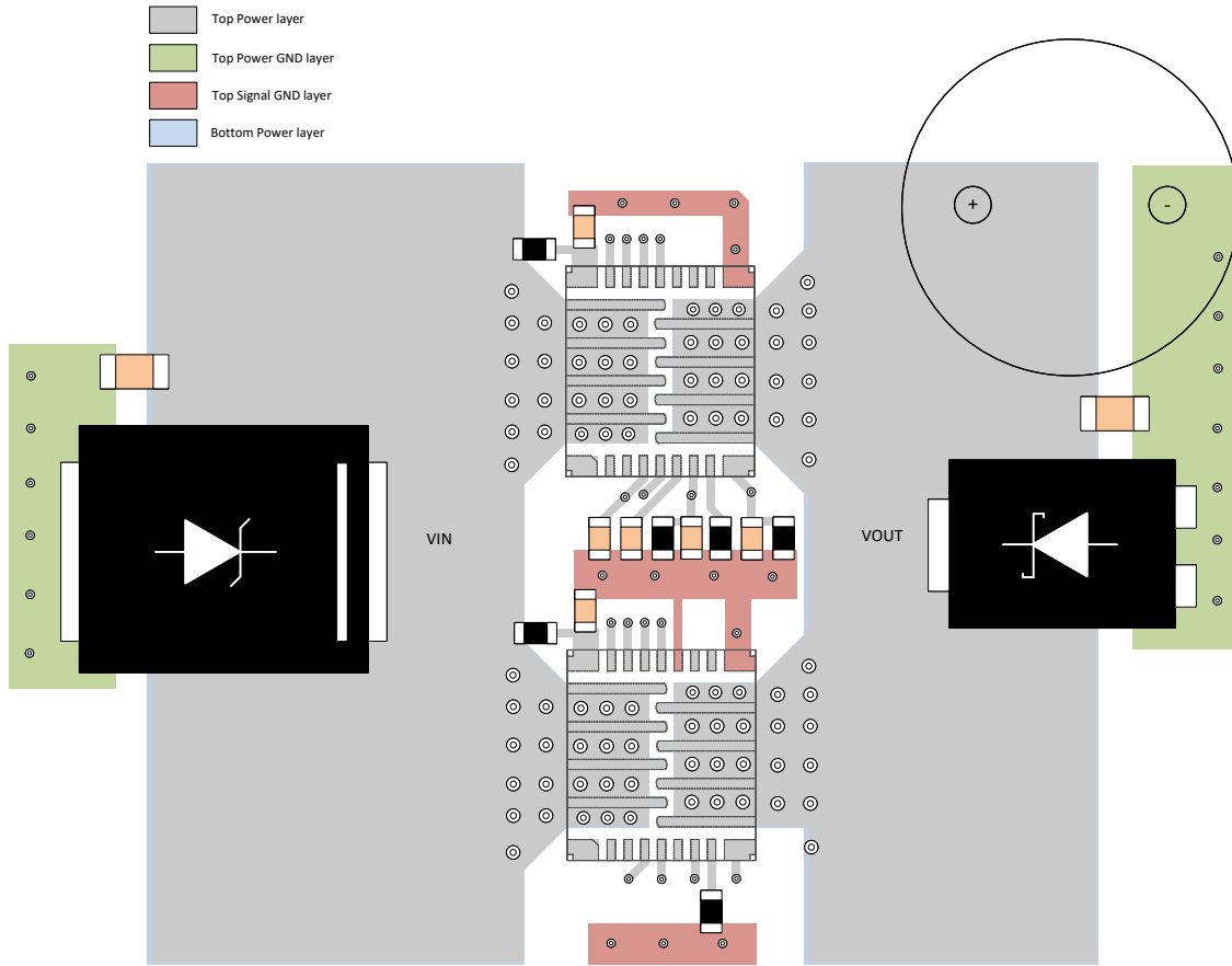
图 11-1. TPS25985x Two Parallel Devices Layout Example
