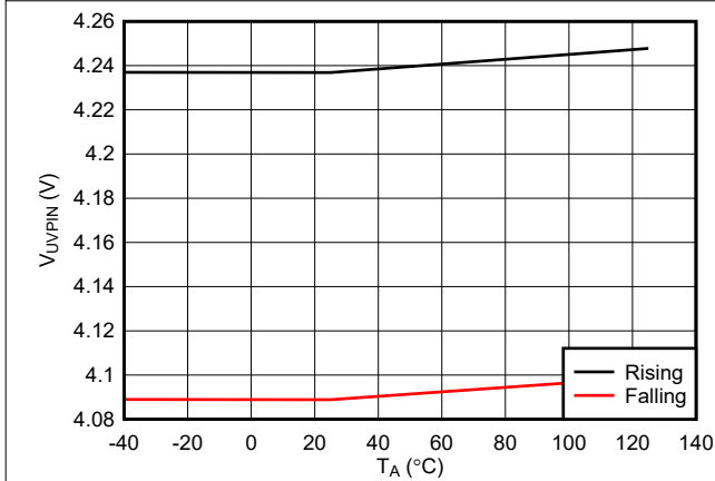
图 7-3. VIN Undervoltage Thresholds Across Temperature
