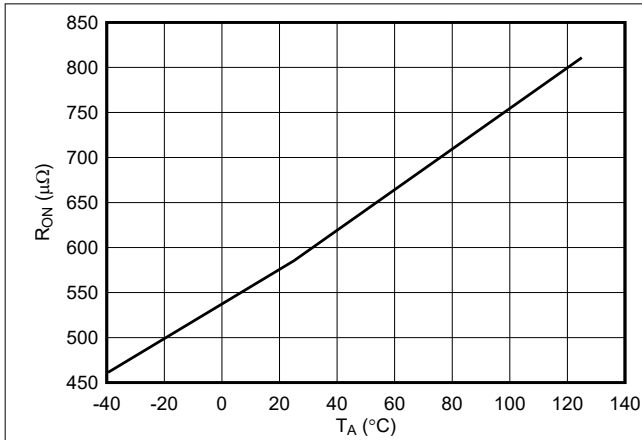
图 7-1. ON Resistance Across Temperature
