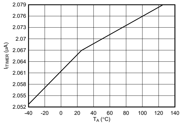
图 7-16. ITIMER Pin Discharge Current Across Temperature
