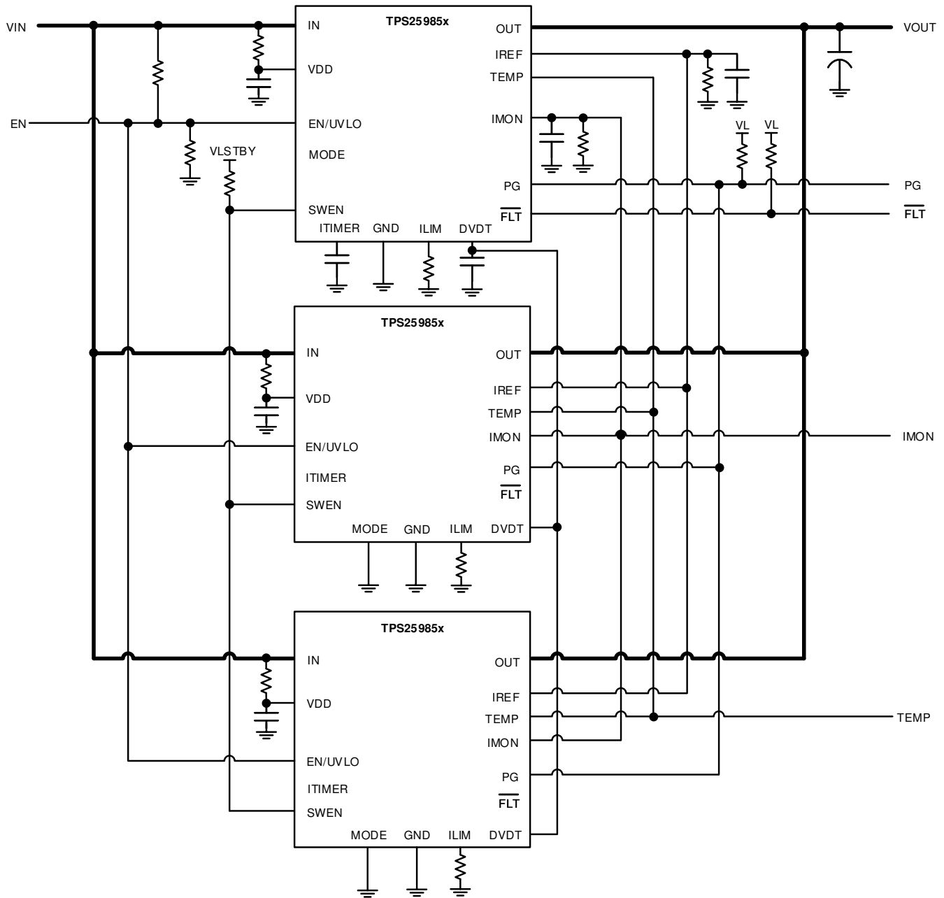
图 9-2. Devices Connected in Parallel for Higher Current Capability
