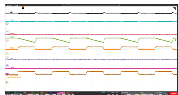
图 9-9. Transient Overload: V_{IN} = 12 V, C_{ITIMER} = 22 nF, C_{LOAD} = 55 mF, R_{IMON} = 167 \Omega , R_{IREF} = 40.2 k \Omega , and Load Current Stepped from 300 A to 400 A then 300 A within 10 ms
