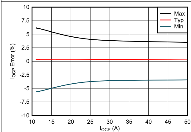
图 7-11. Steady-State Overcurrent Protection Threshold (Circuit-Breaker) Accuracy
