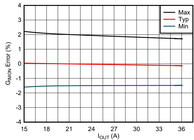
图 7-10. IMON Gain Accuracy Across Process and Temperature Corners
