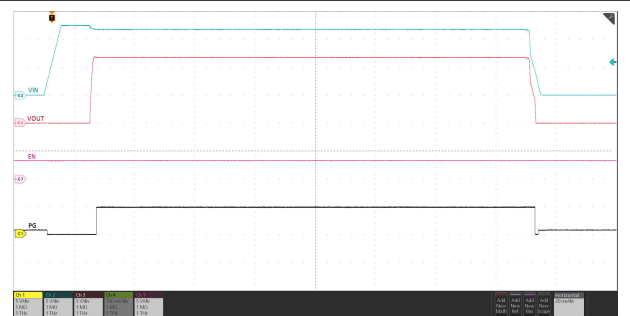
图 7-24. Power Up and Down Sequencing Using Input Supply
