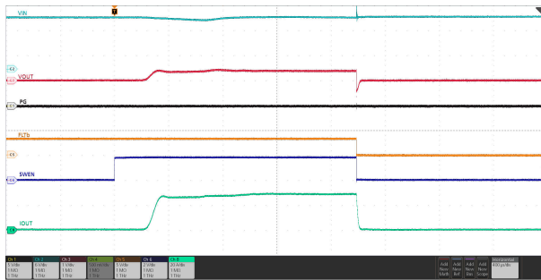
图 7-31. Overcurrent Protection Response (Circuit-Breaker)
