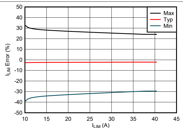
图 7-12. Start-up Overcurrent Protection Threshold (Current Limit) Accuracy
