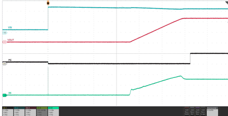
Input supply stepped up from 0 V to 12 V. Device waits for t_{\text{INSDLY}} for input supply to stabilize before it turns on the output.
