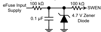
图 9-18. Zener Regulator Used as Pullup Supply for SWEN
