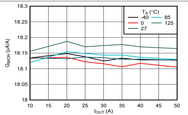
图 7-8. IMON Gain Across Load and Temperature
