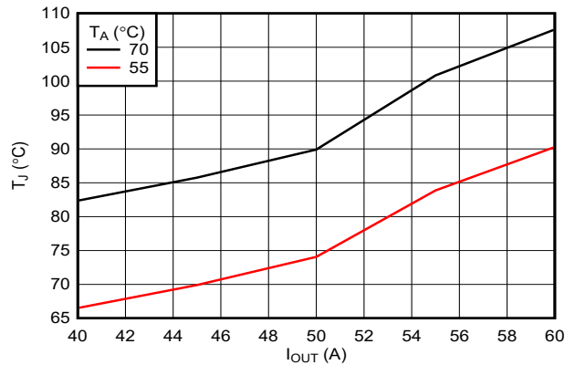
图 7-22. Junction Temperature vs Load Current (No Air-Flow)
