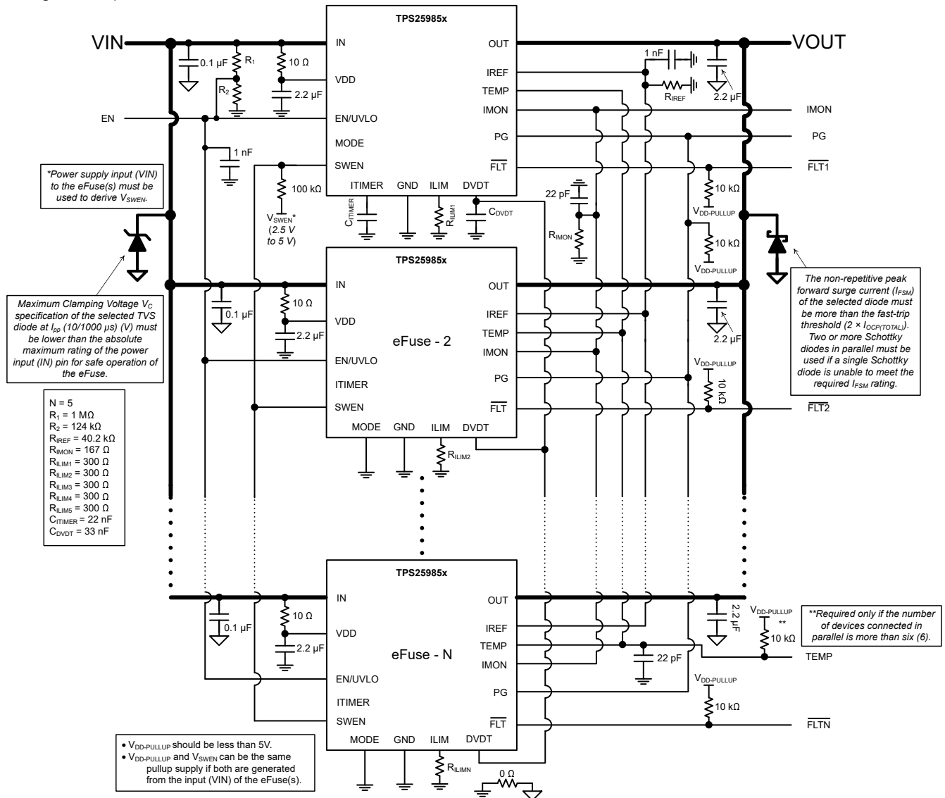
图 9-3. Application Schematic for a 12-V, 3.6-kW Power Path Protection Circuit
