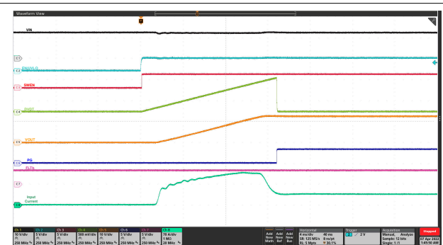
图 9-5. Start-up with EN/UVLO: V_{IN} = 12 V, EN/UVLO Stepped Up From 0 V to 3 V, C_{LOAD} = 55 mF, R_{LOAD(Start-up)} = 0.33 \Omega , C_{DVDT} = 33 nF, R_{IREF} = 40.2 k \Omega , and R_{ILIM} on Each Device = 300 \Omega
