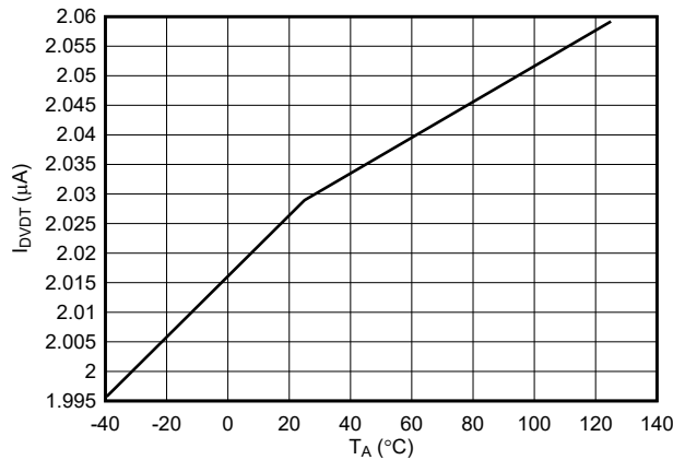
图 7-19. DVDT Charging Current Across Temperature
