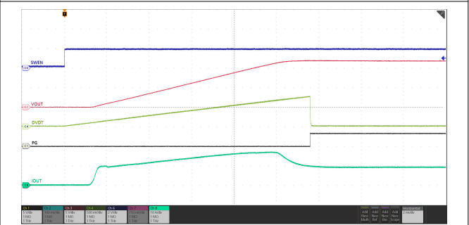
C_{OUT} = 6.8 \text{ mF} , R_{OUT} = 1.2 \Omega , C_{dVdt} = 33 \text{ nF} 图 7-28. Inrush Current Control with Capacitive and Resistive Load
