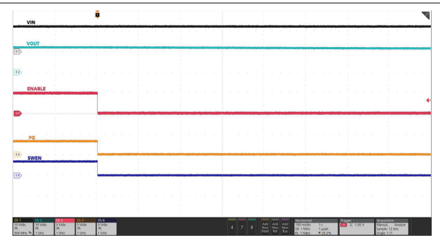
IN supply held steady at 12 V, EN pin toggled from high to low. C_{OUT} = 18\text{ mF} , C_{dVdt} = 33\text{ nF} , I_{LOAD} = 0\text{ A}
