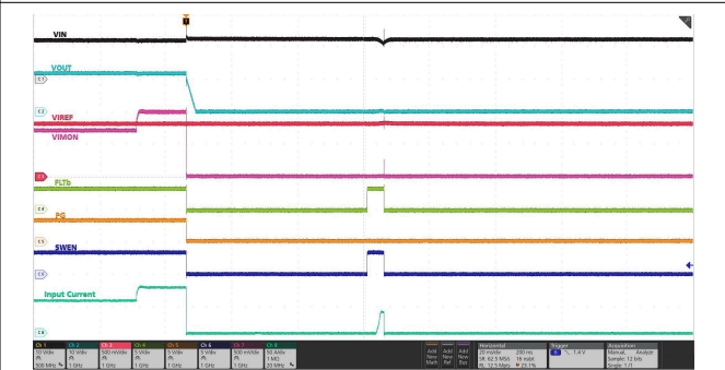
Device in steady-state, Load current ramped up from 50 A to 70 A for 100 ms. OCP threshold set to 55 A, Overcurrent blanking delay set to 15 ms (OC_TIMER = 0x89), Auto-retry 1 times configuration (RETRY_CONFIG[5:3] = 001b), Auto-retry delay set to 55 ms (RETRY_CONFIG[2:0] = 000b)
