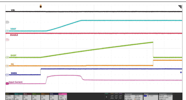
IN supply held steady at 12 V, EN pin held high, PMBus OPERATION ON Command. C_{OUT} = 18\text{ mF} , C_{dVdt} = 33\text{ nF}
