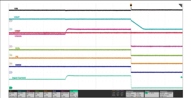
Device in steady-state, Load current ramped up from 50 A to 70 A for > 15 ms. OCP threshold set to 55 A, Overcurrent blanking delay set to 15 ms (OC_TIMER = 0x89)
