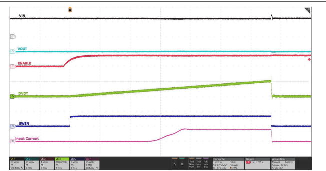
图 7-56. Power Up into Short-Circuit Protection
