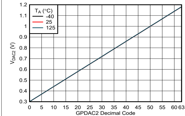
图 7-27. General Purpose DAC2 Transfer Function
