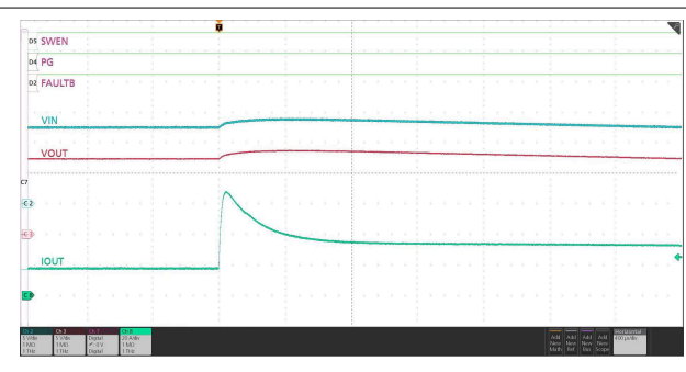
图 7-58. Short-Circuit Protection During Steady-state
