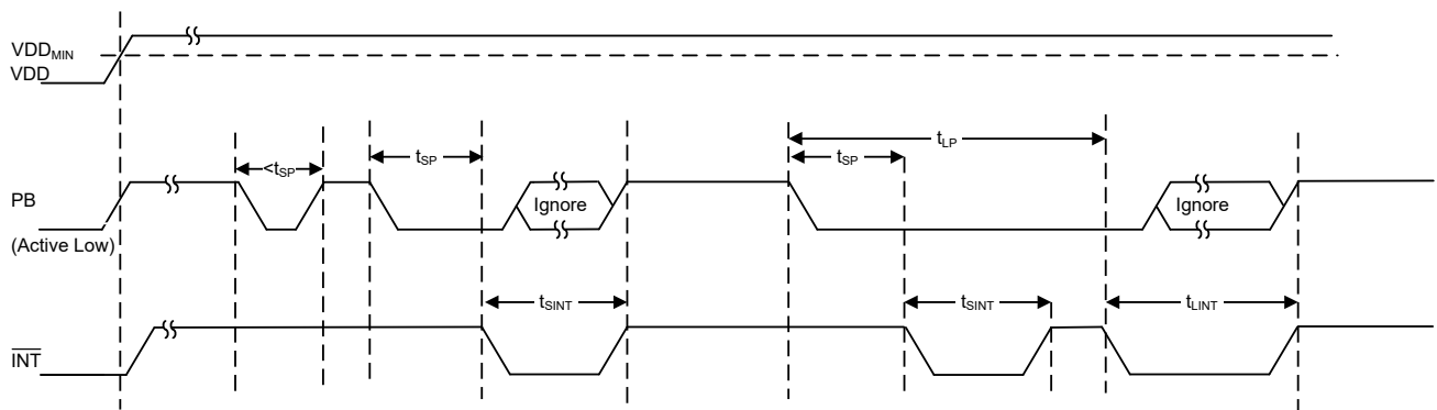
PB input is ignored if it's width is less than t_{sp} . PB input is ignored if it is released and again pressed during interrupt pulse.
