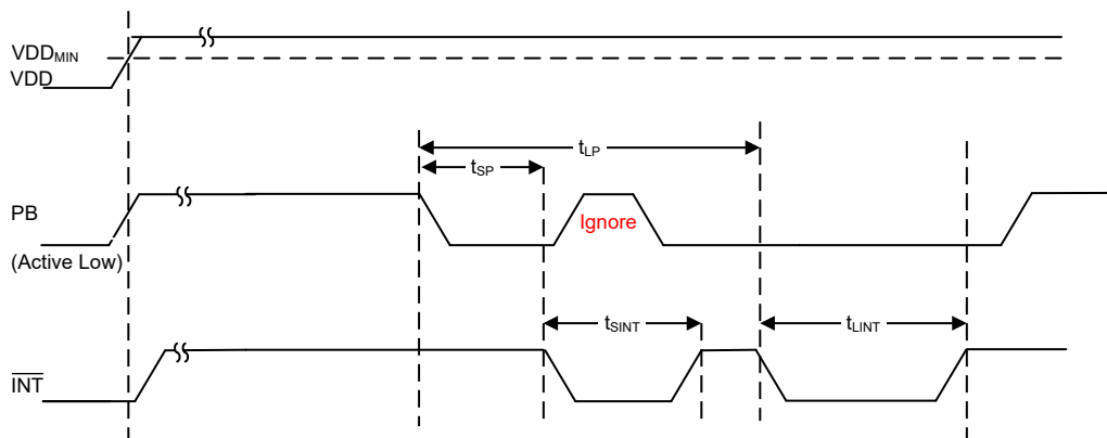
The timer ignores the transition at PB pin during t_{SINT} pulse.
