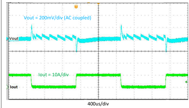
图 8-16. Transient Response, 0 A to 10 A, Slew Rate = 2.5 A/μs
