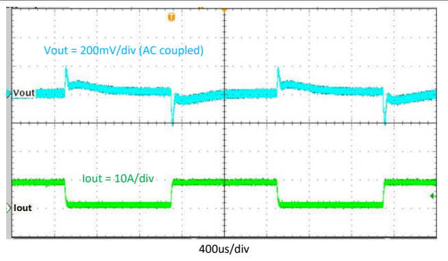
图 8-15. Transient Response, 1 A to 9 A, Slew Rate = 2.5 A/μs
