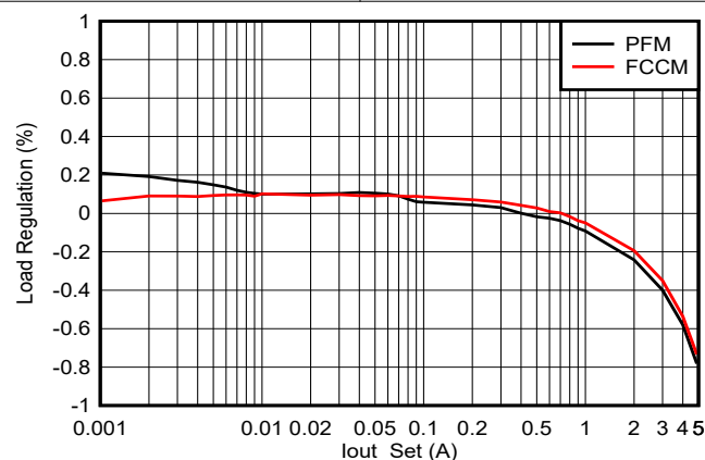
图 5-17. TPS543521 负载调整, V_{IN} = 12\text{V} , V_{OUT} = 3.3\text{V} , f_{SW} = 500\text{kHz}
