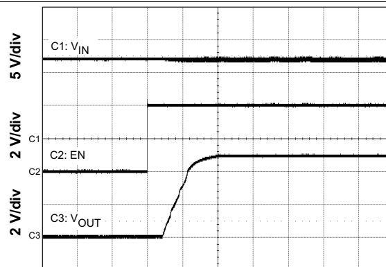
Time = 2 ms/div Figure 38. Startup With EN
