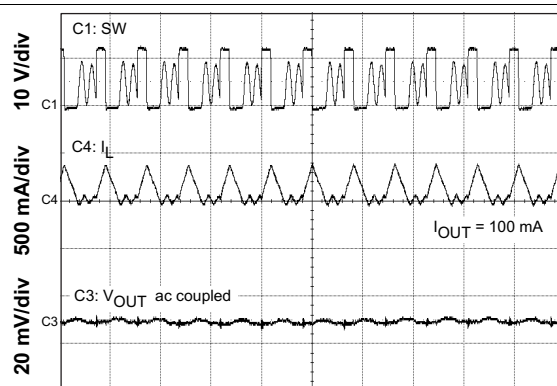
Time = 2 \mu s/div Figure 40. Output Ripple DCM
