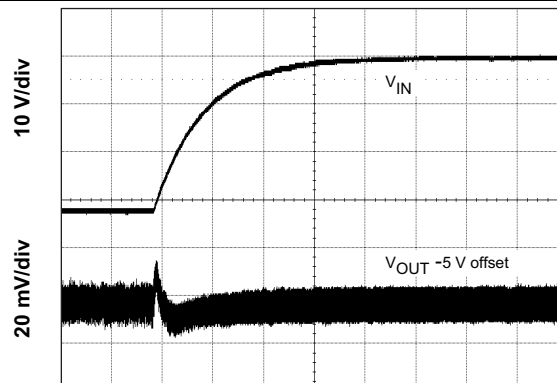
Time = 5 ms/div Figure 36. Line Transient (8 V To 40 V)
