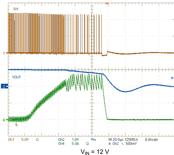
图 8-20. Overcurrent Protection – Overload
