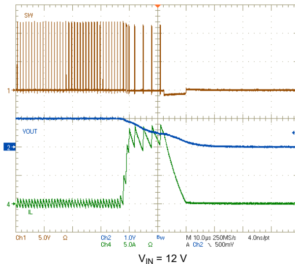
图 8-21. Overcurrent Protection – Short
