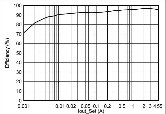
图 5-16. TPS54538 效率 (PFM), V_{IN} = 24\text{V} , V_{OUT} = 12\text{V} , f_{SW} = 500\text{kHz} , L = 5.6\mu\text{H}
