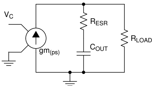
图 7-12. Small Signal Model for Peak Current Mode Control
