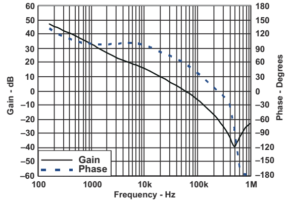
图 8-9. Closed-Loop Response
