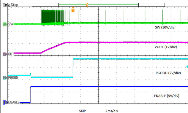
图 6-15. Enable Power Up, Pre-Bias
