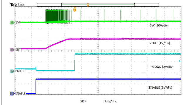
图 8-18. Enable Power Up into Pre-bias, Skip
