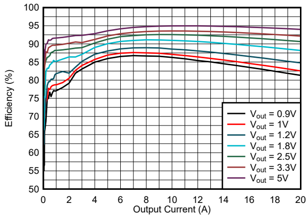
图 6-1. Efficiency vs Output Current, 12 V_{IN} , 800 KHz, DCM, V_{CC} = \text{Int}
