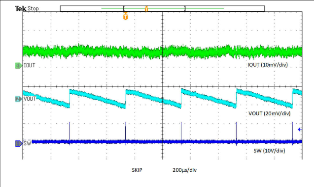
图 6-18. V_{OUT} Ripple, Skip Mode, 10-mA Load
