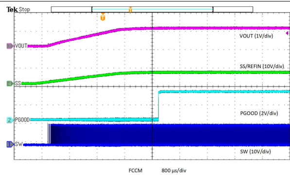
图 8-27. Exiting Overtemperature Protection in FCCM
