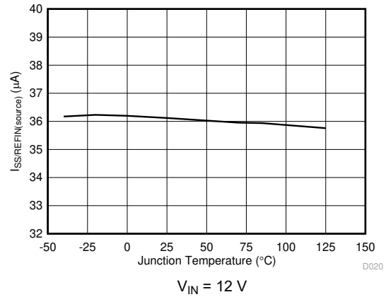
图 6-10. I_{SS}(\text{source}) vs Junction Temperature
