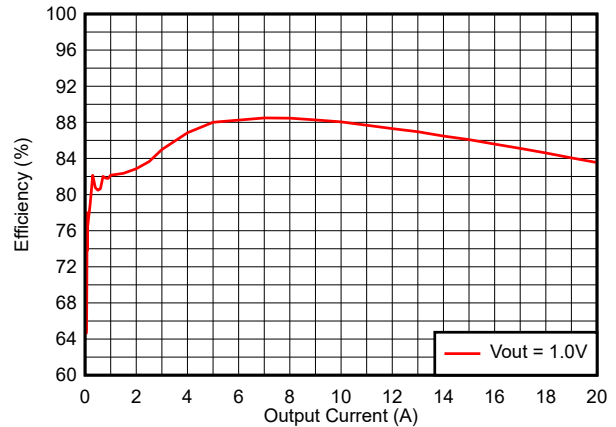
图 8-3. Efficiency vs Output Current, Internal VCC Bias, Skip
