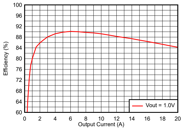
图 8-4. Efficiency vs Output Current, VCC = 3.3-V External Bias, FCCM
