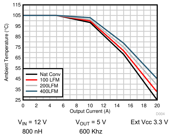
图 6-6. Safe Operating Area, V_{OUT} = 5 \text{ V}
