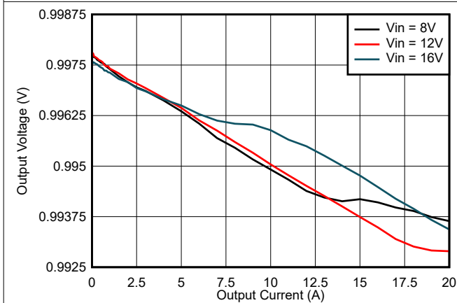
图 8-10. Output Voltage vs Output Current, VCC = 3.3-V External Bias, FCCM
