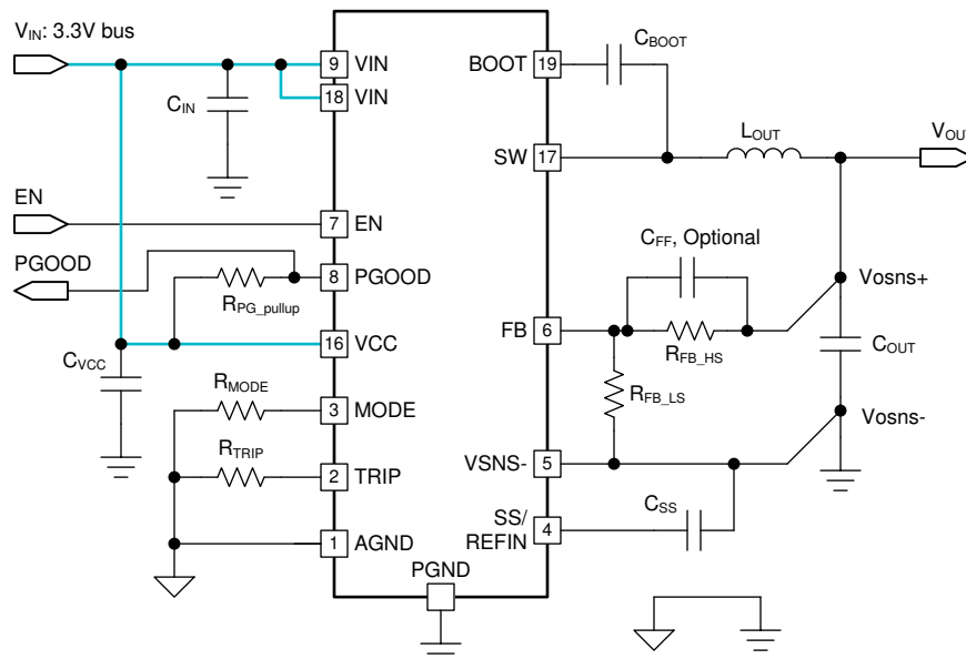
图 7-6. Single V_{IN} Configuration for a 3.3-V Bus
