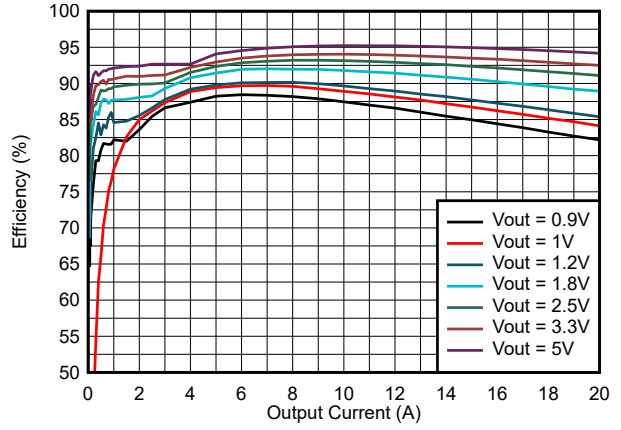
图 6-2. Efficiency vs Output Current, 12 V_{IN} , 800 KHz, DCM, V_{CC} = \text{EXT } 3.3 \text{ V}
