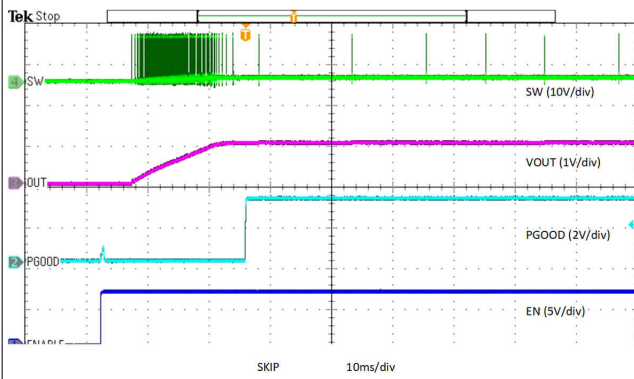
图 6-13. Enable Power Up, Skip
