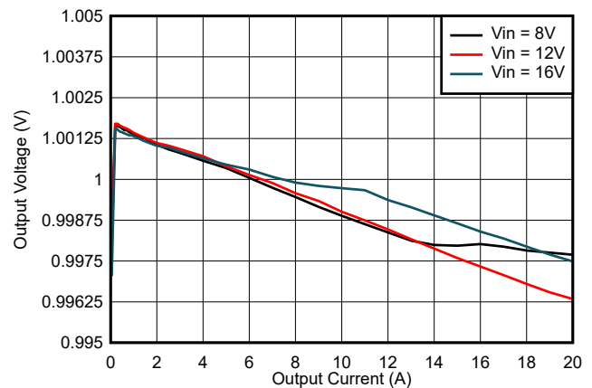
图 8-7. Output Voltage vs Output Current, Internal VCC Bias, Skip
