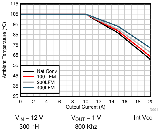
图 6-3. Safe Operating Area, V_{OUT} = 1.0 \text{ V}
