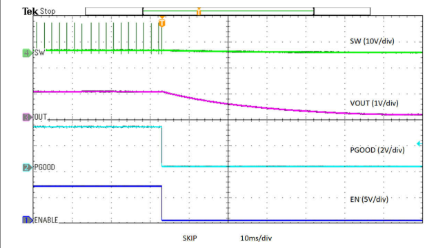
图 8-19. Enable Power Down with Pre-bias, Skip
