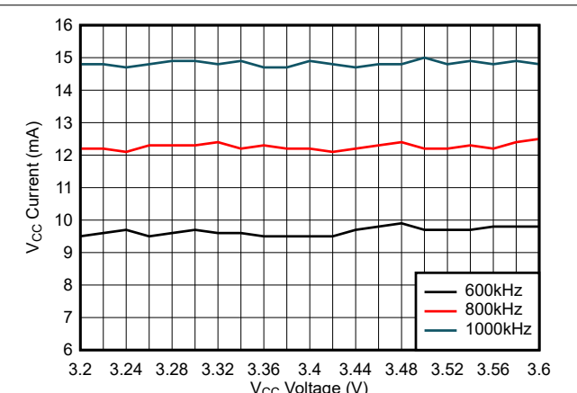
图 8-13. ICC Current vs External VCC Voltage
