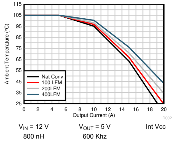
图 6-4. Safe Operating Area, V_{OUT} = 5 \text{ V}
