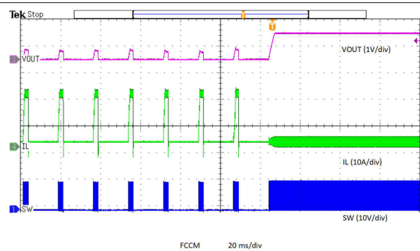
图 8-29. Hiccup Overcurrent
