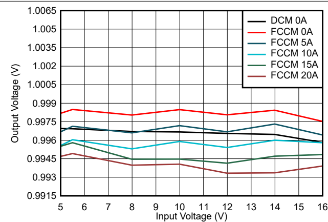
图 8-11. Output Voltage vs Input Voltage, Internal VCC Bias
