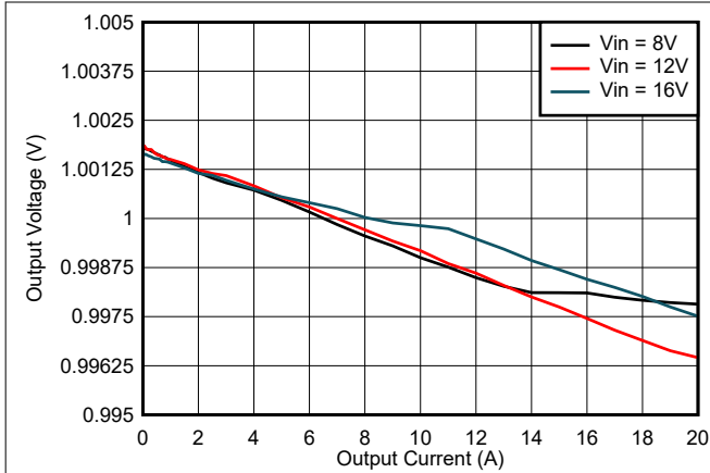
图 8-8. Output Voltage vs Output Current, Internal VCC Bias, FCCM
