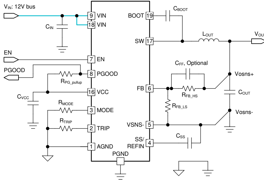
图 7-5. Single V_{IN} Configuration for a 12-V Bus
