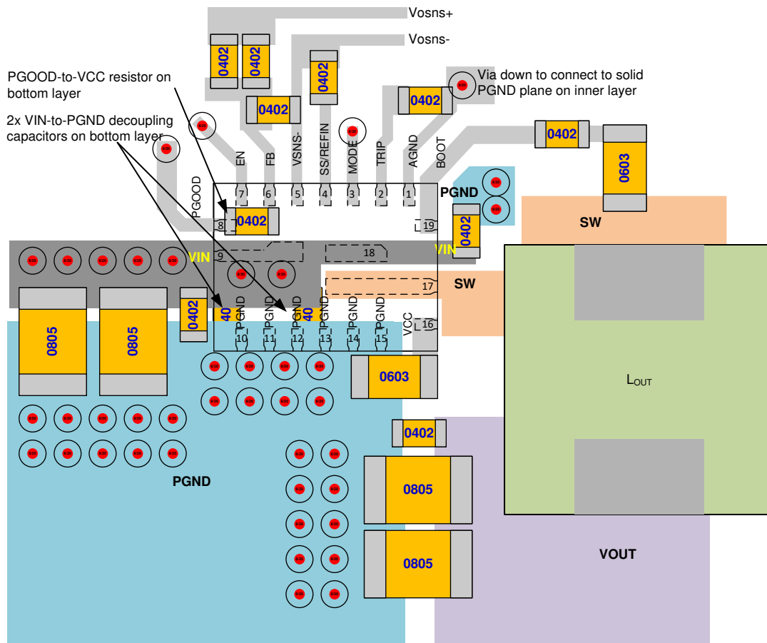
图 10-1. Layout Recommendation
