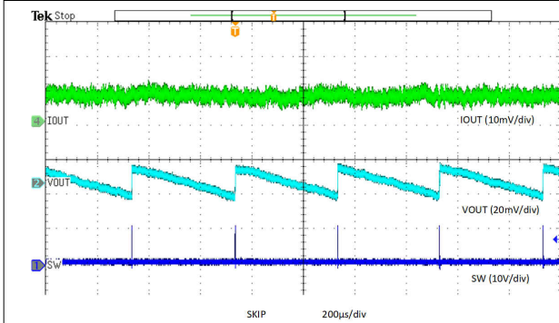
图 8-24. Output Voltage Ripple, Skip, 0.01-A Load
