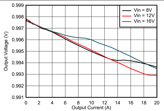
图 8-9. Output Voltage vs Output Current, VCC = 3.3-V External Bias, Skip
