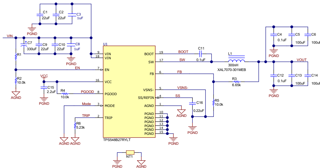
图 8-1. TPS548B27 Application Circuit Diagram
