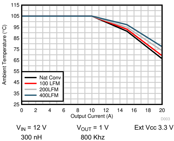
图 6-5. Safe Operating Area, V_{OUT} = 1 \text{ V}
