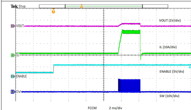
图 8-28. Enabled into Overcurrent
