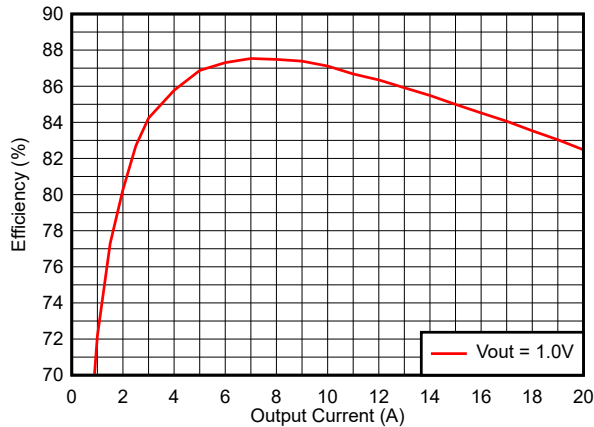
图 8-2. Efficiency vs Output Current, Internal VCC Bias, FCCM
