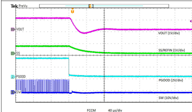
图 8-26. Overtemperature Protection in FCCM
