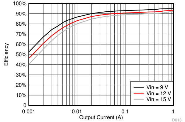
图 6-12. TPS561201 V_{OUT} = 5\text{ V} , Efficiency, L = 4.7\ \mu\text{H}
