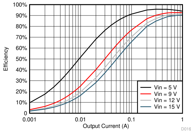
图 6-15. TPS561208 V_{OUT} = 3.3\text{ V} , Efficiency, L = 3.3\ \mu\text{H}
