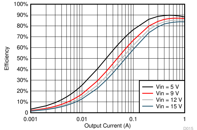
图 6-14. TPS561208 V_{OUT} = 1.5\text{ V} , Efficiency, L = 2.2\ \mu\text{H}
