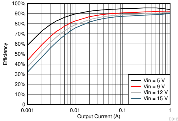
图 6-11. TPS561201 V_{OUT} = 3.3\text{ V} , Efficiency, L = 3.3\ \mu\text{H}
