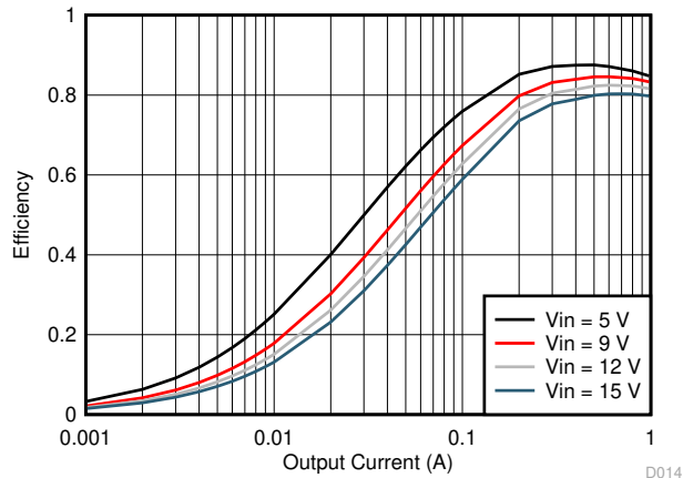
图 6-13. TPS561208 V_{OUT} = 1.05\text{ V} , Efficiency, L = 2.2\ \mu\text{H}
