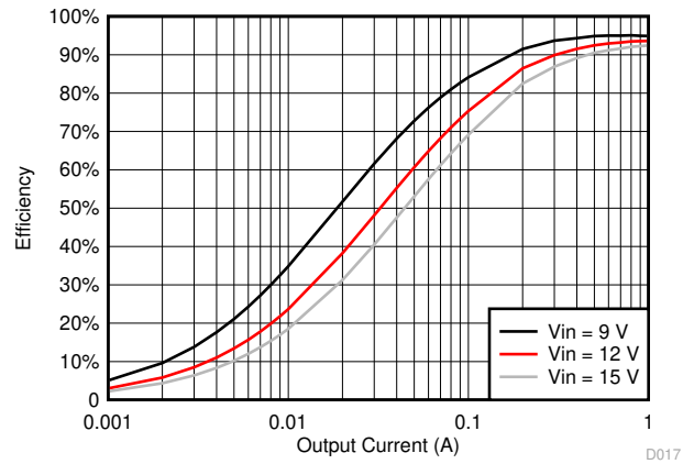
图 6-16. TPS561208 V_{OUT} = 5\text{ V} , Efficiency, L = 4.7\ \mu\text{H}
