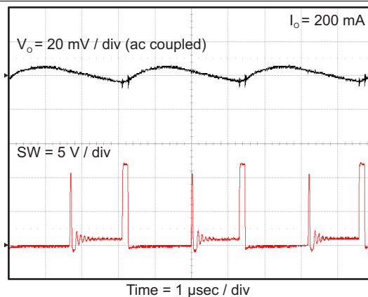
Figure 26. TPS562210 Output Voltage Ripple
