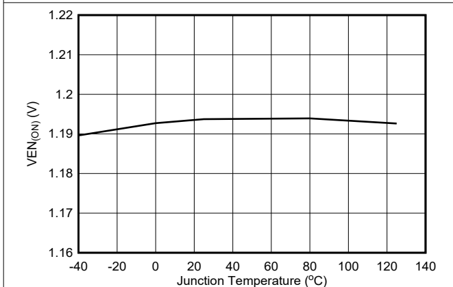
图 6-3. Enable On Threshold Voltage
