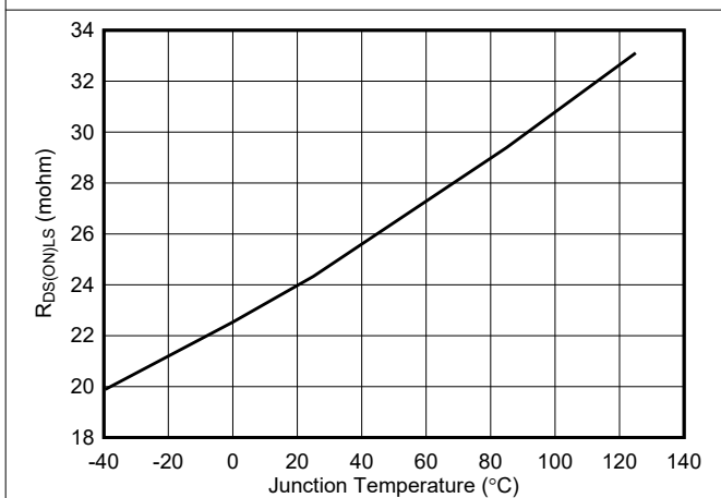
图 6-5. Low-Side R_{DS(ON)}
