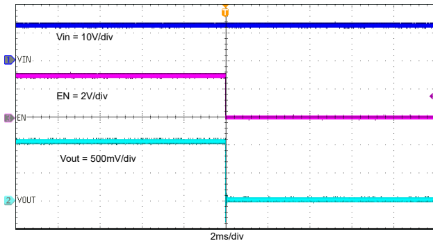
图 8-16. Shutdown Through EN, I_{OUT} = 3 A
