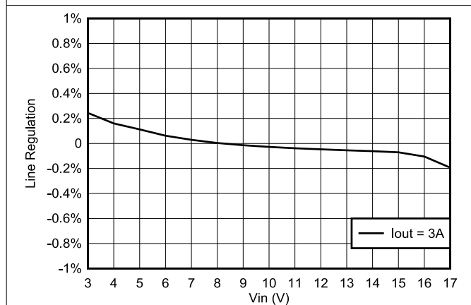
图 8-6. TPS563252 Line Regulation vs V_{IN}
