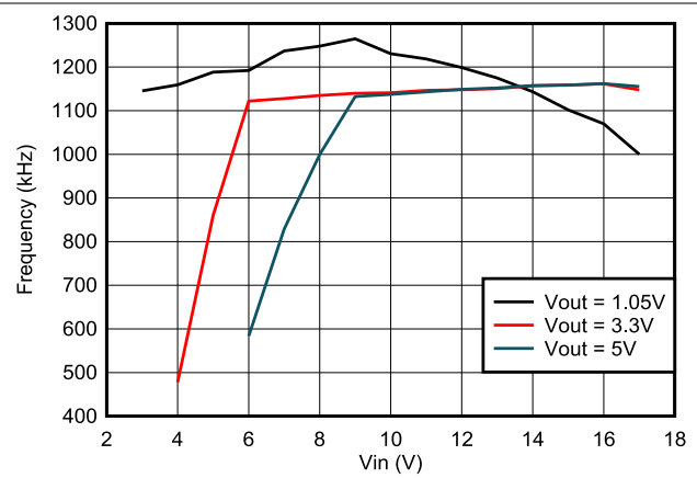
图 6-8. Frequency vs Input Voltage, I_{OUT} = 3\text{ A}
