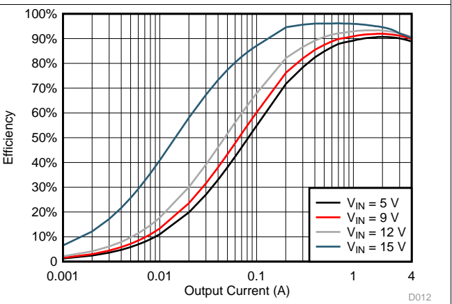
Figure 10. TPS564208 V_{OUT} = 1.5\text{ V} Efficiency, L = 2.2\ \mu\text{H}
