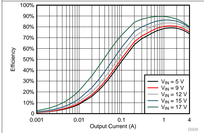
Figure 9. TPS564208 V_{OUT} = 1.05\text{ V} Efficiency, L = 2.2\ \mu\text{H}
