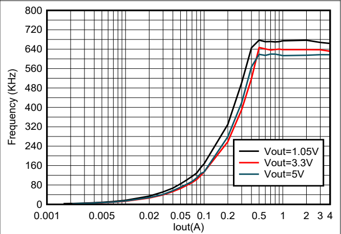
图 6-10. TPS564252 Frequency vs Loading, V_{IN} = 12\text{ V}
