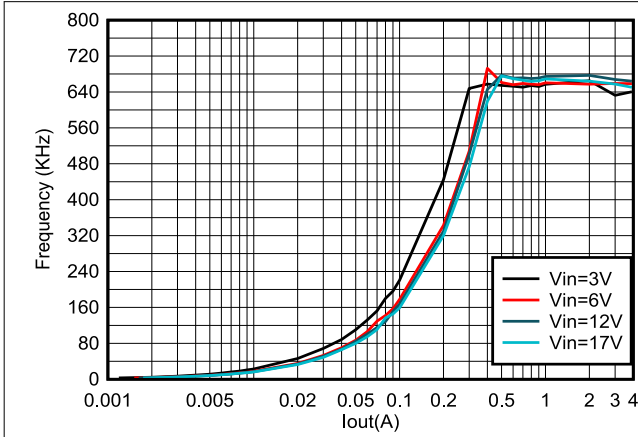
图 8-2. TPS564252 Frequency vs Loading
