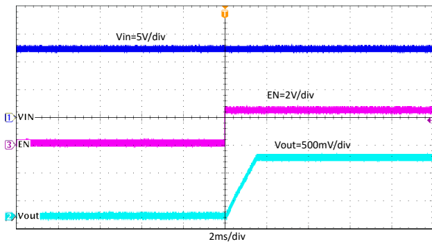
图 8-18. Start-Up Through EN, I_{OUT} = 4 A
