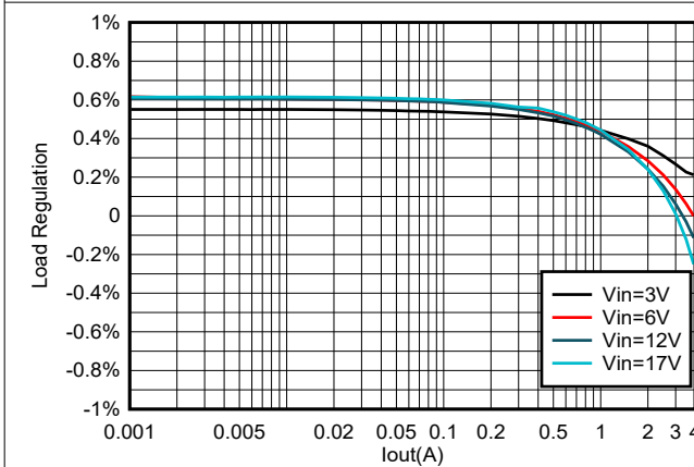
图 8-6. TPS564257 Load Regulation vs Loading
