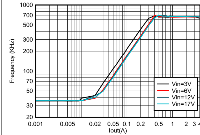
图 8-4. TPS564255 Frequency vs Loading
