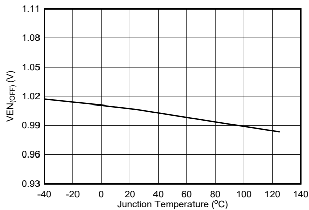
图 6-5. Enable Off Threshold Voltage
