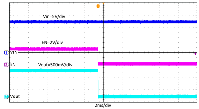
图 8-19. Shutdown Through EN, I_{OUT} = 4 A
