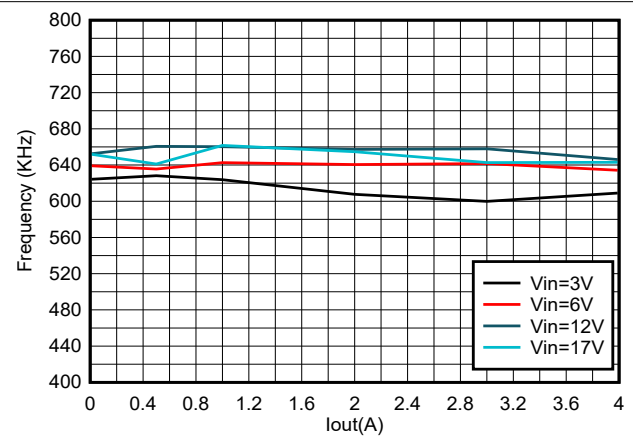
图 8-3. TPS564257 Frequency vs Loading
