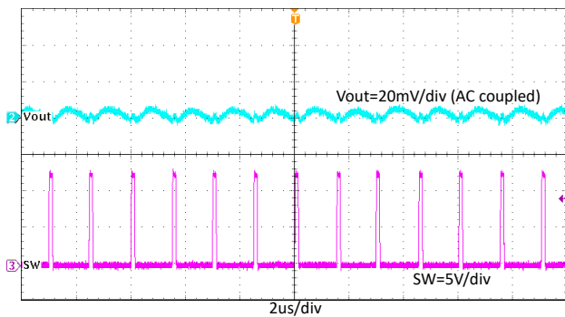
图 8-12. TPS564257 Output Voltage Ripple with 0.01-A Loading
