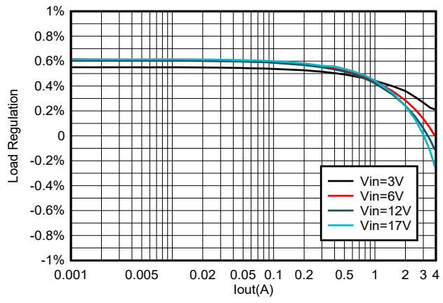
图 8-5. TPS564252 Load Regulation vs Loading
