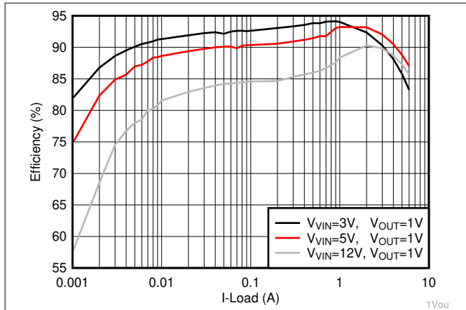
图 7-2. TPS566231 Efficiency Curve
