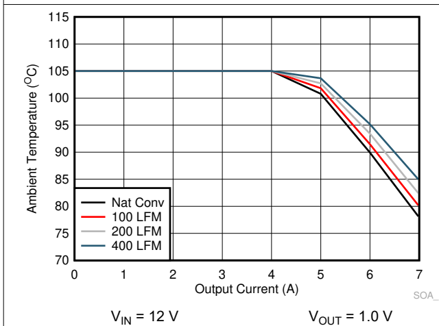
图 5-17. Safe Operating Area
