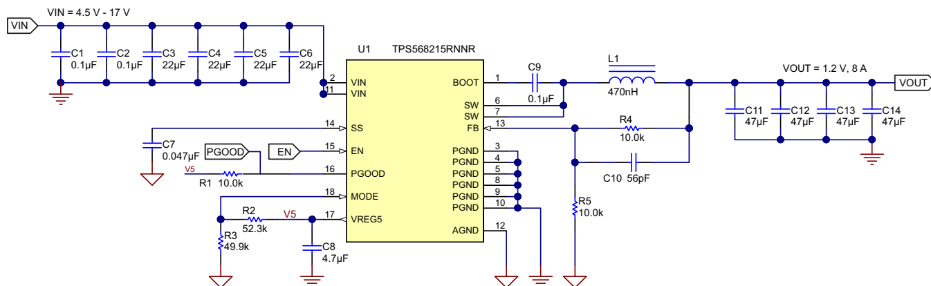
图 22. Application Schematic
