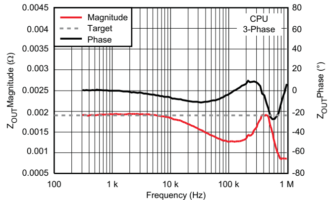
Figure 18. Output Impedance
