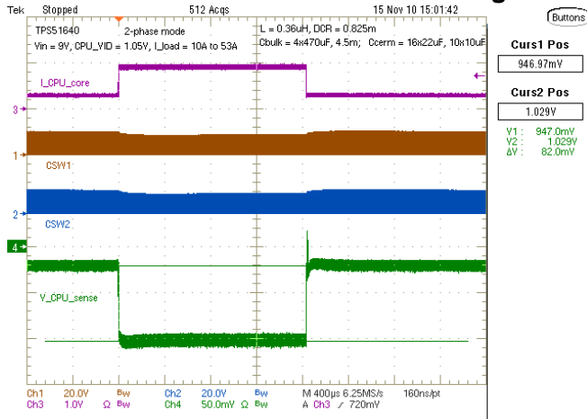
Figure 25. Load Transient, V_{IN} = 9V , Load Step = 43 A
