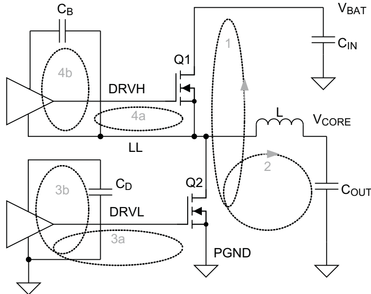
Figure 73. Major Current Loops to Minimize
