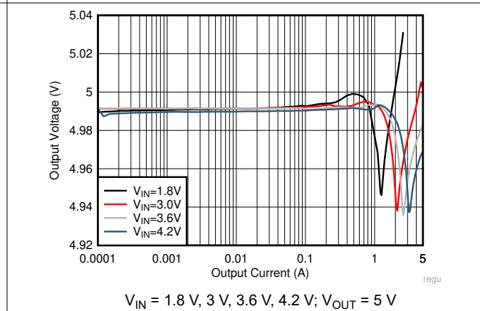
图 6-6. Load Regulation in Forced PWM
