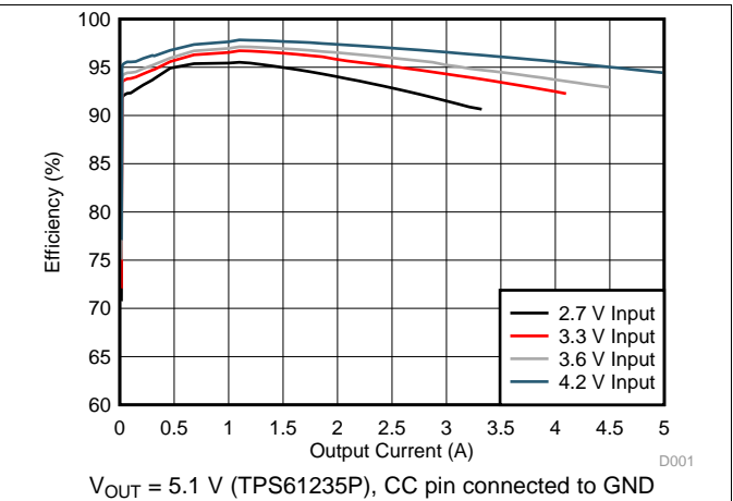
Figure 2. Efficiency vs Output Current with Different Inputs
