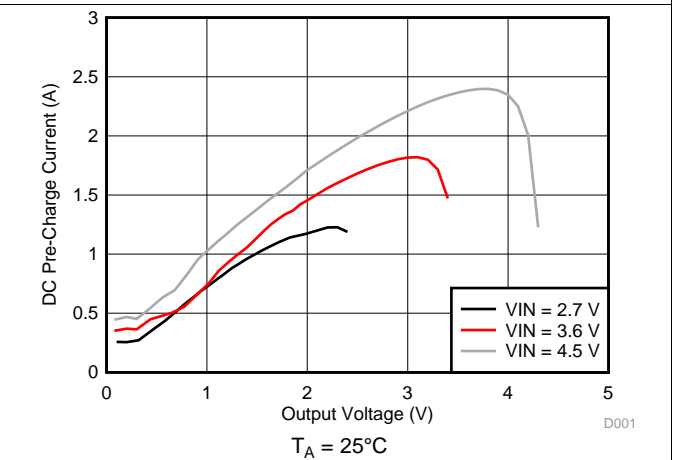
Figure 6. DC Pre-Charge Current vs Output Voltage
