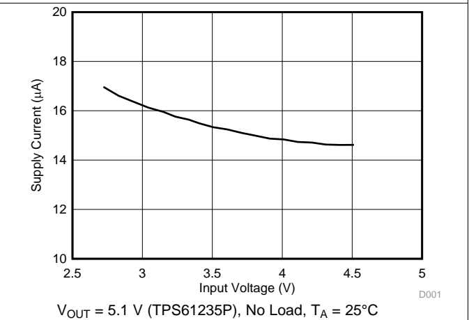
Figure 4. No Load Supply Current vs Input Voltage
