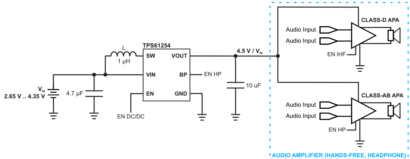
Figure 38. Combined Audio Amplifier Power Supply
