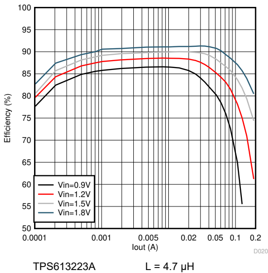
图 6-9. Load Efficiency with Different Inputs
