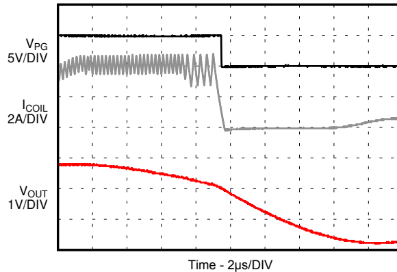
图 8-34. HICCUP Short-Circuit Protection
