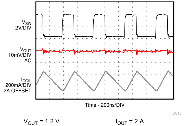
图 9-15. Output Ripple, PWM Operation (2.0 MHz)
