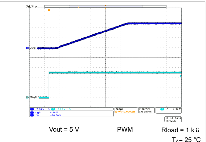
图 10-58. Start-Up Timing
