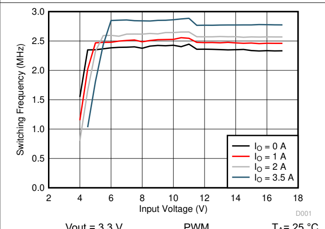
图 10-72. Switching Frequency vs Input Voltage
