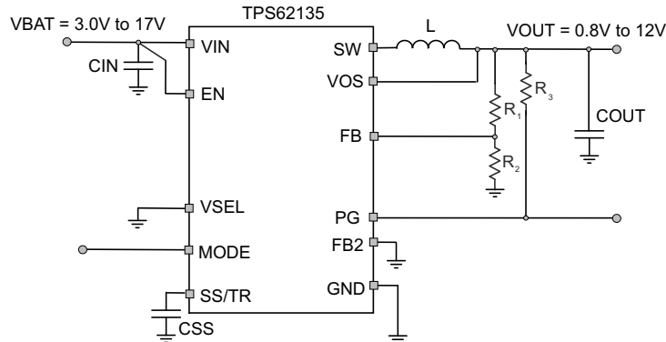
图 8-1. Measurement Setup
