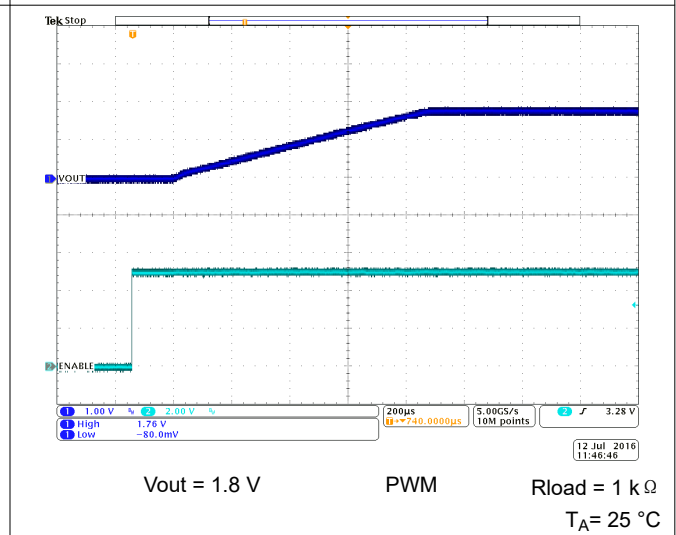
图 10-44. Start-Up Timing
