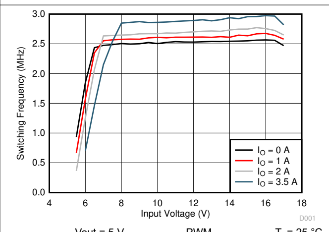
图 10-74. Switching Frequency vs Input Voltage
