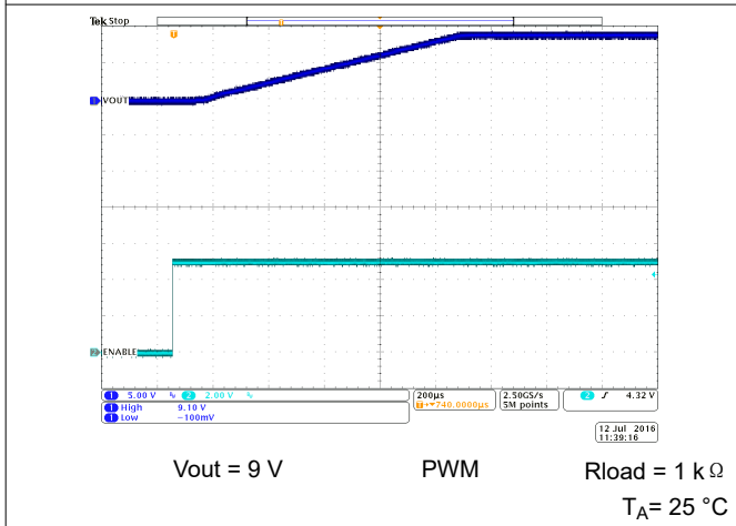
图 10-65. Start-Up Timing
