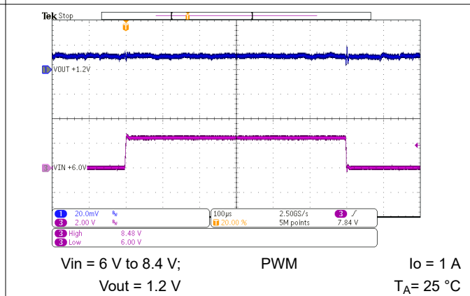
图 10-36. Line Transient Response
