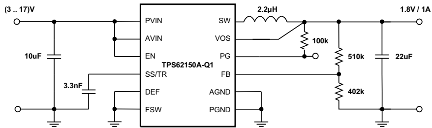
Figure 46. 1.8V/1A Power Supply
