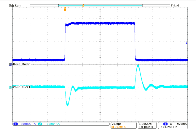
V_{OUT} = 0.6\text{ V} PWM T_A = 25^\circ\text{C} V_{IN} = 3.3\text{ V} I_{OUT} = 0.2\text{ A to } 1.8\text{ A to } 0.2\text{ A}
