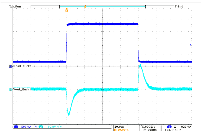
图 10-23. Load Transient Response
