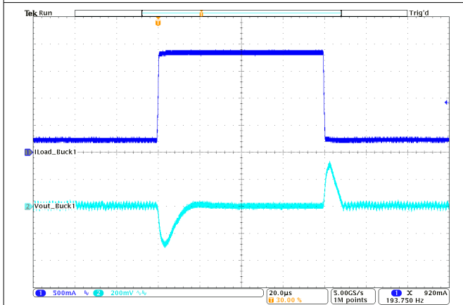
图 10-20. Output Voltage Versus Output Current
