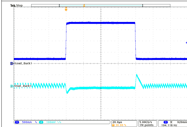
V_{OUT} = 0.6\text{ V} PFM T_A = 25^\circ\text{C} V_{IN} = 3.3\text{ V} I_{OUT} = 0.2\text{ A to } 1.8\text{ A to } 0.2\text{ A}
