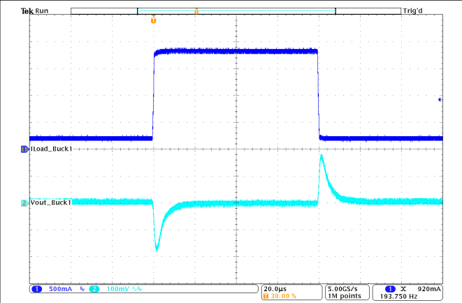
V_{OUT} = 1.0\text{ V} PWM T_A = 25^\circ\text{C} V_{IN} = 5.0\text{ V} I_{OUT} = 0.2\text{ A to } 1.8\text{ A to } 0.2\text{ A}
