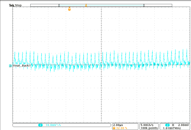
V_{OUT} = 3.3\text{ V} PWM T_A = 25^\circ\text{C} I_{OUT} = 3\text{ A} V_{IN} = 5.0\text{ V} BW = 20\text{ MHz}
