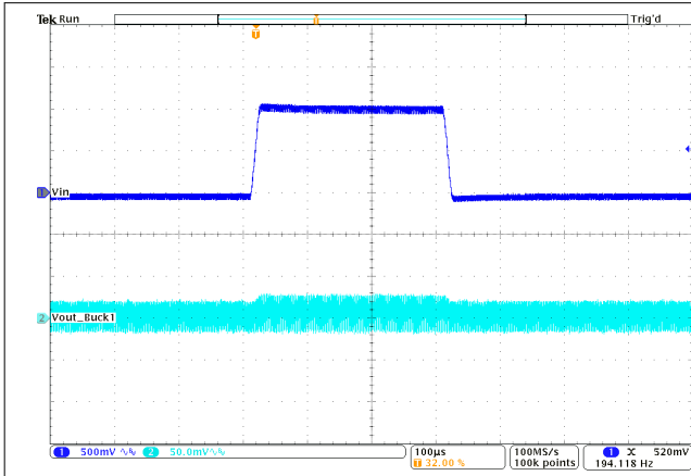
V_{OUT} = 1.0\text{ V} PFM T_A = 25^\circ\text{C} I_{OUT} = 0.3\text{ A} V_{IN} = 4.5\text{ V to } 5.5\text{ V to } 4.5\text{ V}
