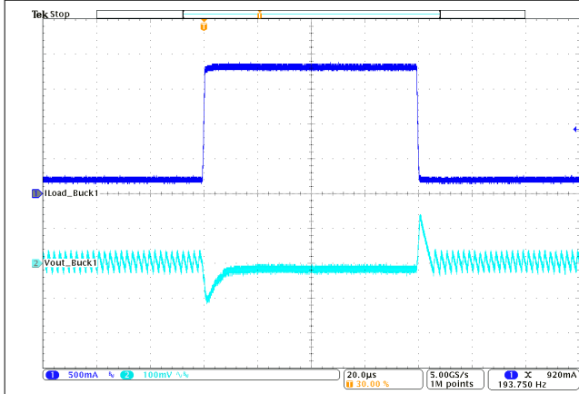
V_{OUT} = 1.0\text{ V} PFM T_A = 25^\circ\text{C} V_{IN} = 5.0\text{ V} I_{OUT} = 0.2\text{ A to } 1.8\text{ A to } 0.2\text{ A}
