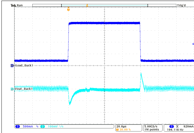
V_{OUT} = 1.2\text{ V} PFM T_A = 25^\circ\text{C} V_{IN} = 5.0\text{ V} I_{OUT} = 0.2\text{ A to } 1.8\text{ A to } 0.2\text{ A}
