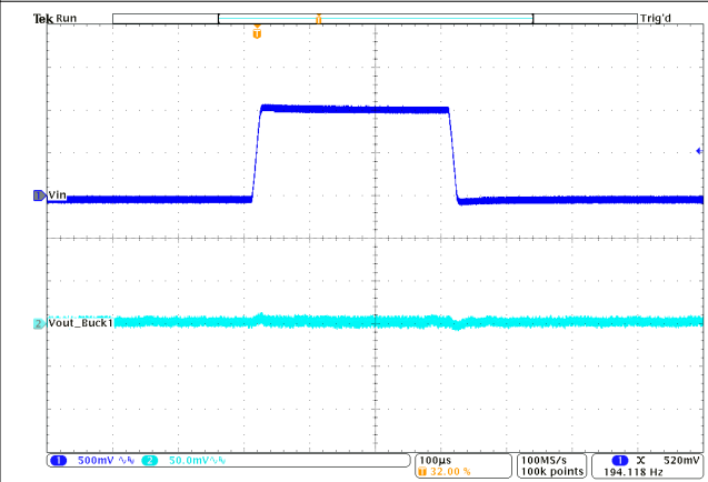
图 10-35. Line Transient Response
