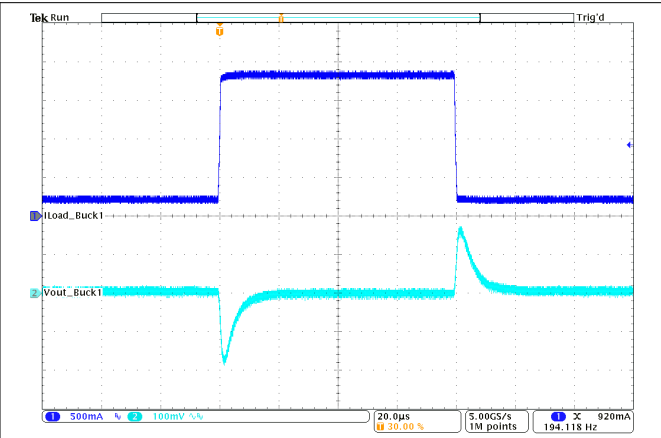
V_{OUT} = 1.2\text{ V} PWM T_A = 25^\circ\text{C} V_{IN} = 5.0\text{ V} I_{OUT} = 0.2\text{ A to } 1.8\text{ A to } 0.2\text{ A}
