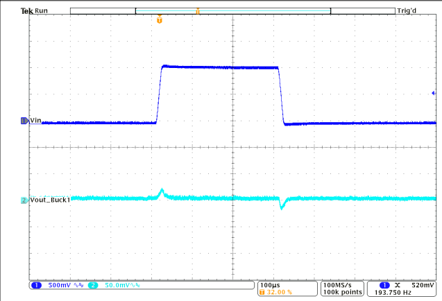
V_{OUT} = 0.6\text{ V} PWM T_A = 25^\circ\text{C} I_{OUT} = 3\text{ A} V_{IN} = 4.5\text{ V to } 5.5\text{ V to } 4.5\text{ V}
