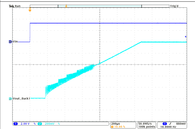
图 10-47. Start-Up Timing
