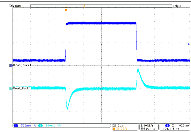
图 10-27. Load Transient Response
