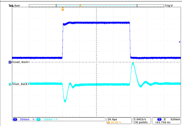
图 10-29. Load Transient Response
