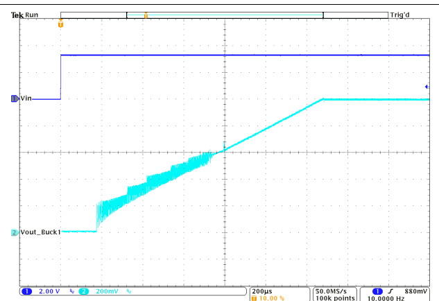
图 10-47. Start-Up Timing
