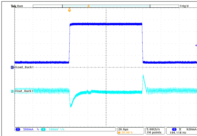
图 10-26. Load Transient Response
