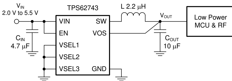
图 9-1. TPS62743 Typical Application Circuit
