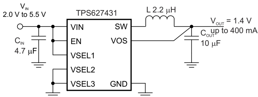
图 9-2. TPS627431 Typical Application Circuit
