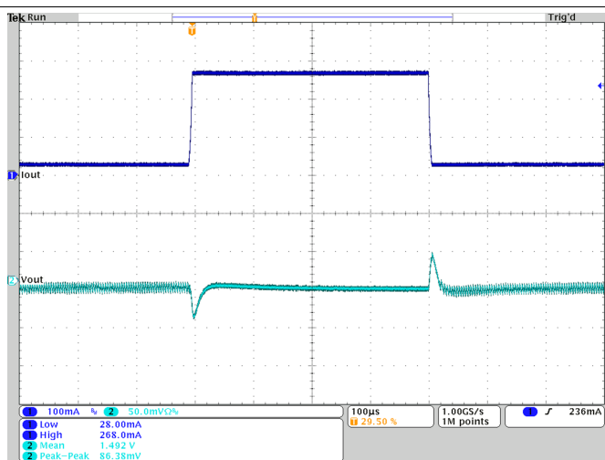
Figure 29. Load Transient Response; V_{OUT} = 1.5 V
