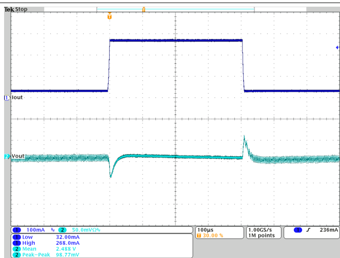
Figure 27. Load Transient Response; V_{OUT} = 2.5 V
