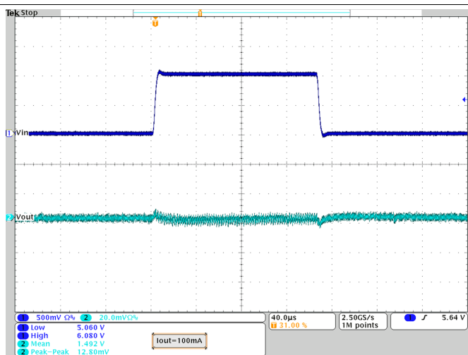
Figure 25. Line Transient Response; V_{OUT} = 1.5 V
