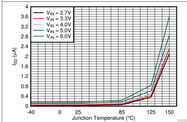
图 7-3. Shutdown Current vs Temperature
