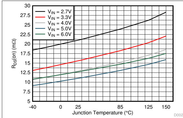
图 7-1. R_{DS(ON)} of High-Side Switch
