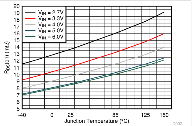
图 7-2. R_{DS(ON)} of Low-Side Switch
