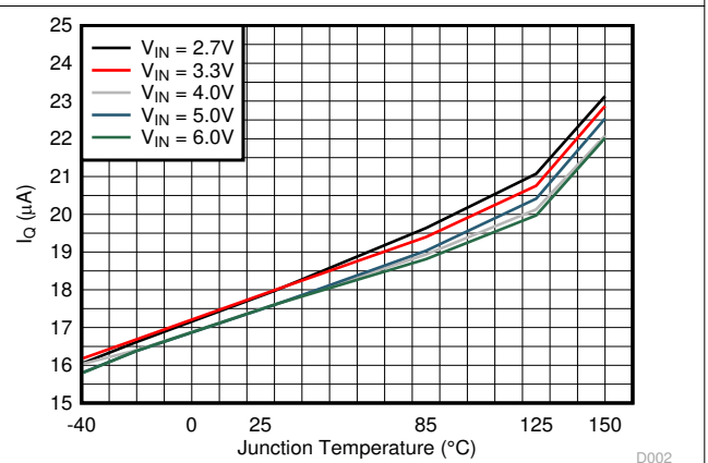
图 7-4. Quiescent Current vs Temperature
