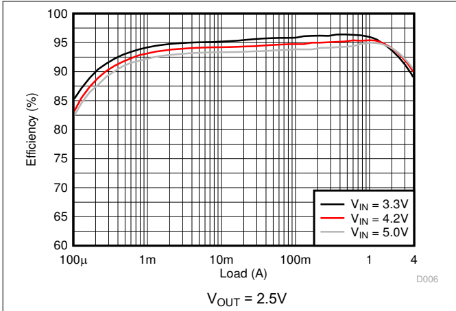
图 8-15. Efficiency
