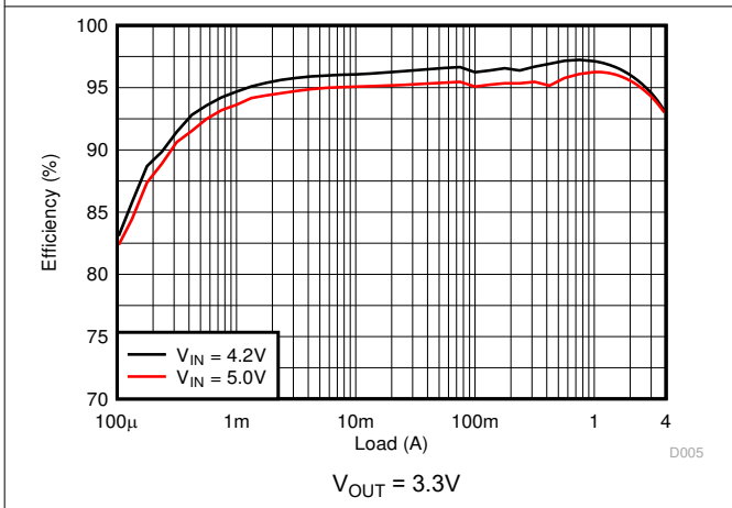
图 8-19. Efficiency
