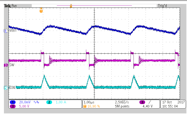
I_{OUT} = 0.1A TPS62824/5/6/7
